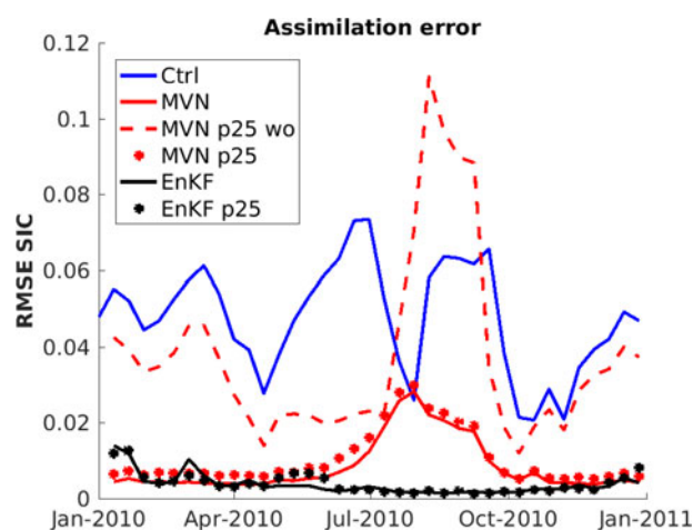
Fig. 7. RMSE of SIC after assimilation of SIC for 2010. For the dotted lines, only 25% of the SIC observations were used for the assimilation. The red and black dots are the MVN- and EnKF-assimilated runs, respectively. The dashed, red line, the MVN assimilation without spatial extrapolation was used for assimilation of 25% of the SIC observations. The solid lines show assimilation using all observations, the blue line is the control model, the red line is the MVN model, and the black line is the EnKF model.
