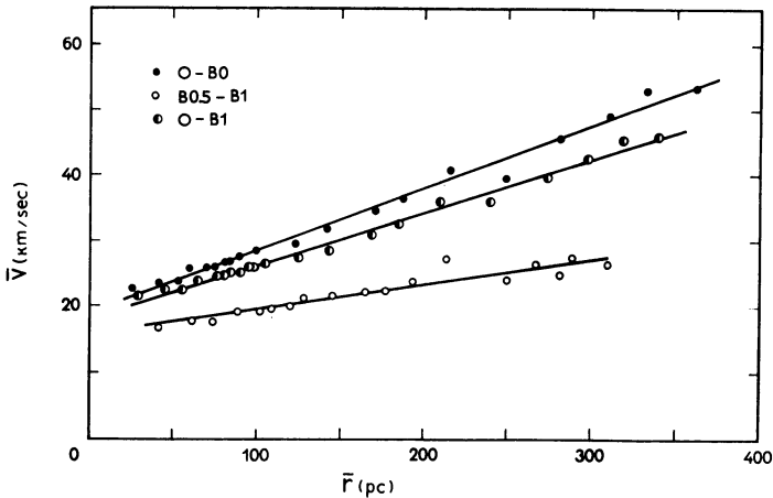
Fig. 1. The dependence \bar{V}(\bar{r}) in the synthetic association: for O-B0 (full dots), B0.5-B1 (open circles) and O-B1 (semifilled circles) stars. The lines are the solutions by the least-square method.
