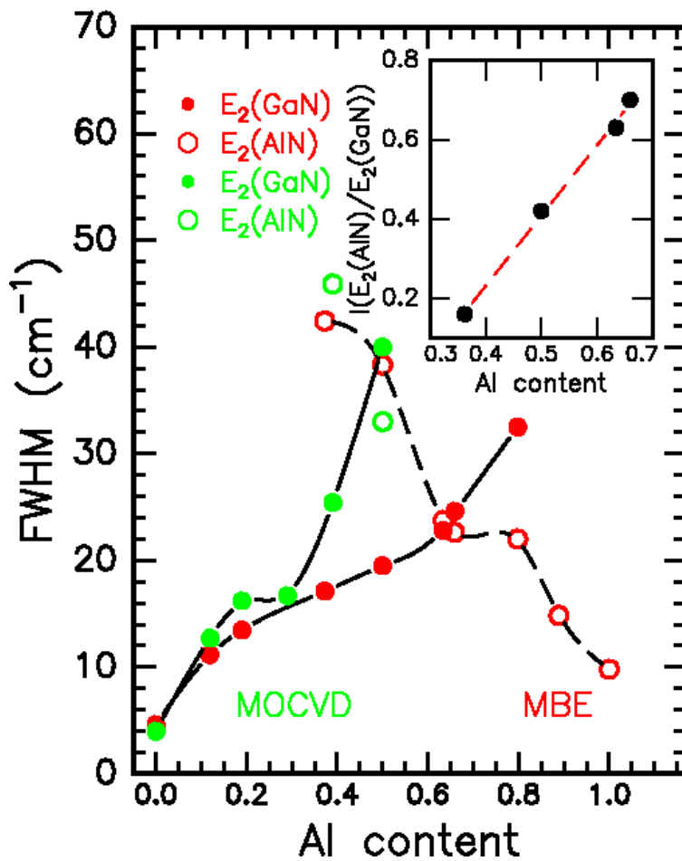
Figure 5. Dependence of the linewidths of the E 2 (GaN) (full dots) and E 2 (AlN) (empty dots) phonon modes on aluminum content for the MBE (red) and MOCVD (green) samples. The lines are drawn as guides to the eyes. The inset shows the relative intensities of the E 2 (GaN) and E 2 (AlN) phonon modes as a function of aluminum content
