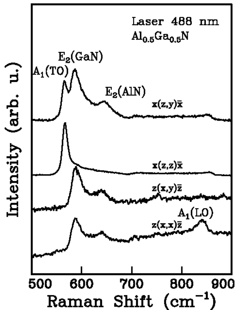
Figure 1. Room temperature Raman spectra of an \text{Al}_x\text{Ga}_{1-x}\text{N} sample with a thickness of 3\mu\text{m} and an aluminum content of 50%. The polarization configuration used is indicated on each spectrum.
