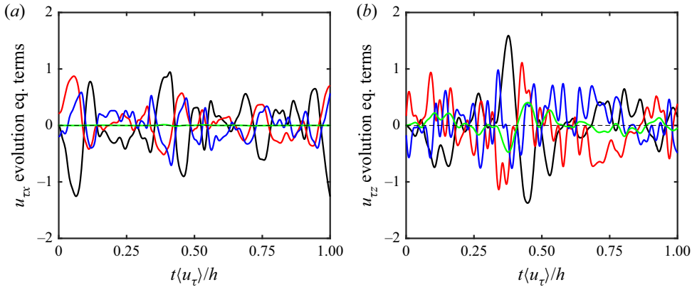
Figure 7. Time signals of terms in the evolution equation for u_\tau , (2.14) at some arbitrary representative point at the wall from LES or channel flow at Re_\tau = 1000 and \Delta/h = 1/30 . Time signals shown are for the terms \partial u_\tau / \partial t (black), V_\tau \cdot \nabla_h u_\tau (red), -T_s^{-1}[u_\tau^{-1}(-\Delta \nabla_h \bar{p} / \rho + \bar{\tau}_\Delta) - u_\tau] (blue) and -u_\tau(\delta_\Delta^* / \Delta) \partial \bar{s} / \partial t (green).
