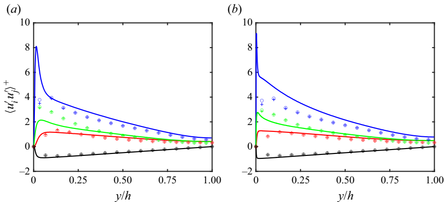
Figure 5. Mean Reynolds stresses for (a) Re_\tau = 1000 and (b) Re_\tau = 5200 . Colours correspond to \langle u'u' \rangle^+ (blue), \langle v'v' \rangle^+ (red), \langle w'w' \rangle^+ (green) and \langle u'v' \rangle^+ (black). Open circles: WMLES using the new wall model with LaRTE and laminar non-equilibrium parts. Plus signs: WMLES using the EQWM. Lines: DNS from Lee & Moser (2015).
