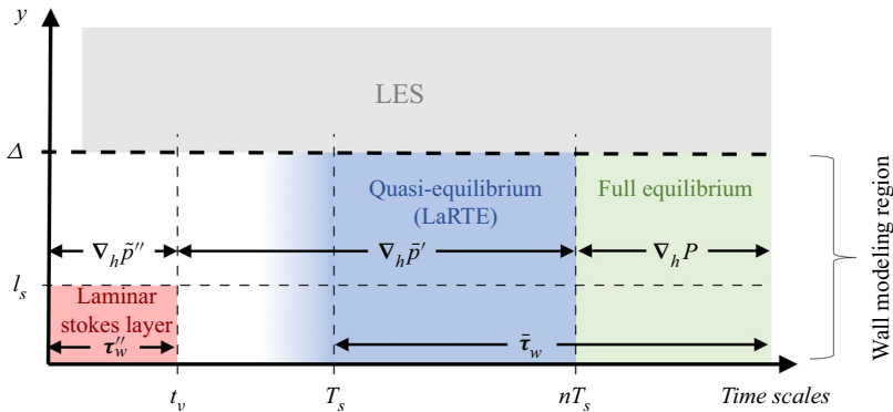
Figure 3. Schematic of the various time scales and wall-normal distances considered for modelling. Different coloured regions identify the corresponding wall modelling components.
