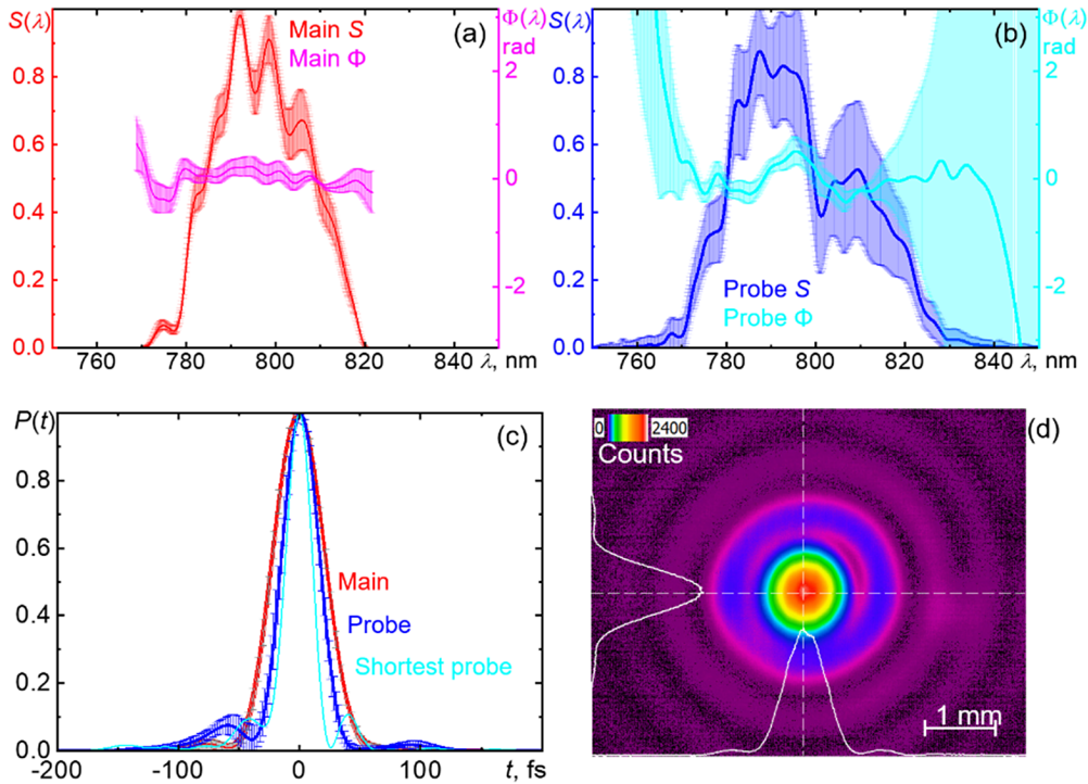
Figure 2. Main and probe pulses before the experiment. (a)–(c) Power amplifier (PA) mode, 1000-shot average for the main and probe pulses, where the error bars are standard deviations of shot-to-shot variations. (a) Red is the main pulse spectrum, while magenta is the main pulse spectral phase. (b) Blue is the probe pulse spectrum, while cyan is probe pulse spectral phase. (c) Red and blue are the main and probe pulse shapes, while cyan is the shortest probe pulse. (d) Down-collimated probe beam spatial profile measured before the fused silica plates by using a low-power infrared laser diode alignment beam.
