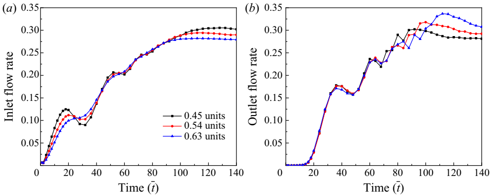
Figure 12. Comparison of (a) inlet flow rate, and (b) outlet flow rate for a gas pocket located at different axial positions for \delta = 4 \times 10^{-4} , \mu_r = 200 and Re_{ss} = 743.4 , while a gas pocket volume of 10 % is considered.
