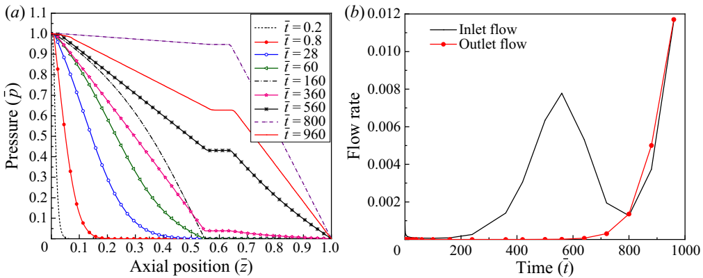
Figure 10. (a) Time evolution of pressure profile as a function of axial position, (b) time evolution of inlet and outlet volumetric flow rates for \delta = 4 \times 10^{-4} , \mu_r = 20\,000 and Re_{ss} = 743.4 , while a gas pocket volume of 10% (the position of the gas pocket is located between 0.55 and 0.64 units from inlet) is considered.
