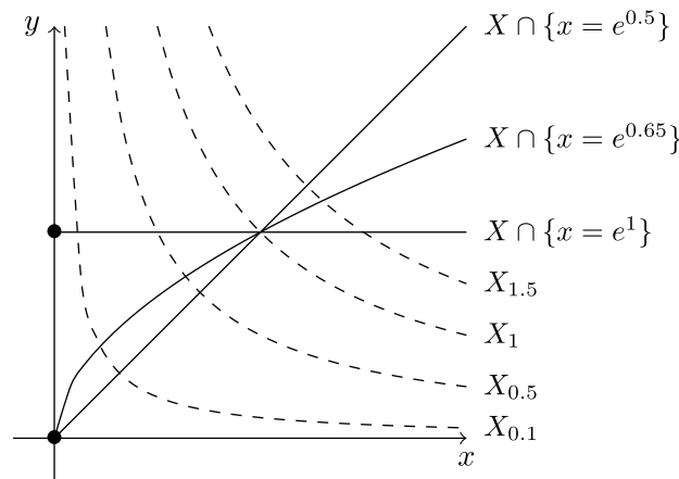
FIGURE 2. The different families in Example 23.
