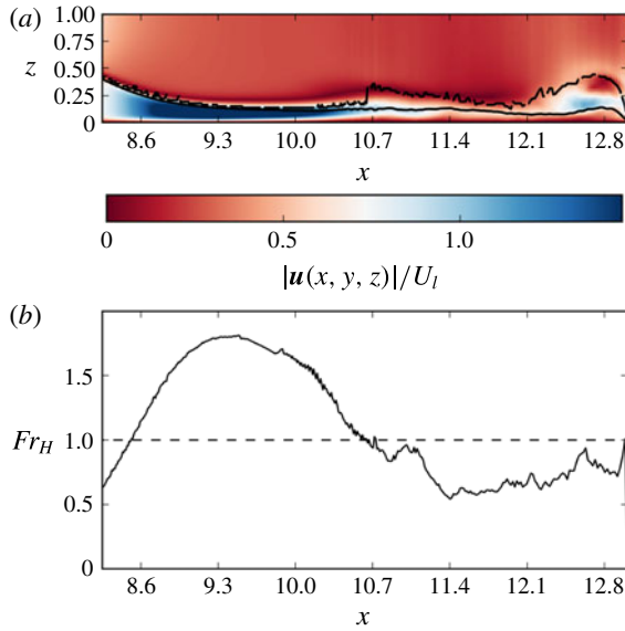
FIGURE 9. (a) Non-dimensional velocity |\mathbf{u}|/U_l on the mid-plane y = y_0 ; the thick black line indicates the depth h_l = \overline{g'h}/g' and the dashed line marks h_i , i.e. the interface \rho = 3\% , (b) Froude number Fr_H versus x . Case S3, t = 16 .
