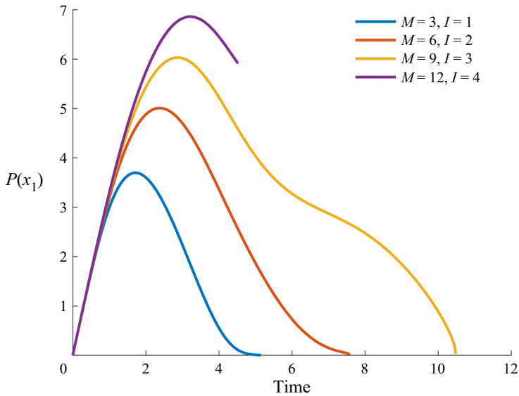
Figure 3. Evolution of the pressure on the body at the moving contact point x_1 as a function of time for varying M = 3I , I = 1, 2, 3, 4 . See table 1 for the other parameter values. The solution curves here terminate at the times when either exiting or flooding occurs.
