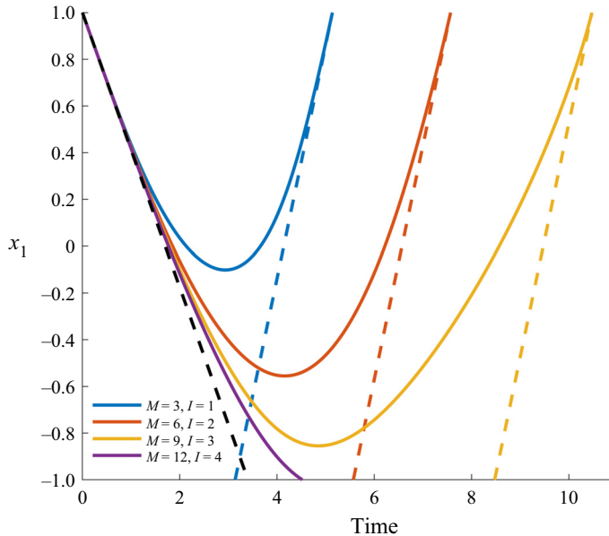
Figure 2. Evolution of x_1 as a function of time for varying M = 3I, I = 1, 2, 3, 4 . The linear behaviours at small times and for exit (dashed lines) are shown. See table 1 for the other parameter values.
