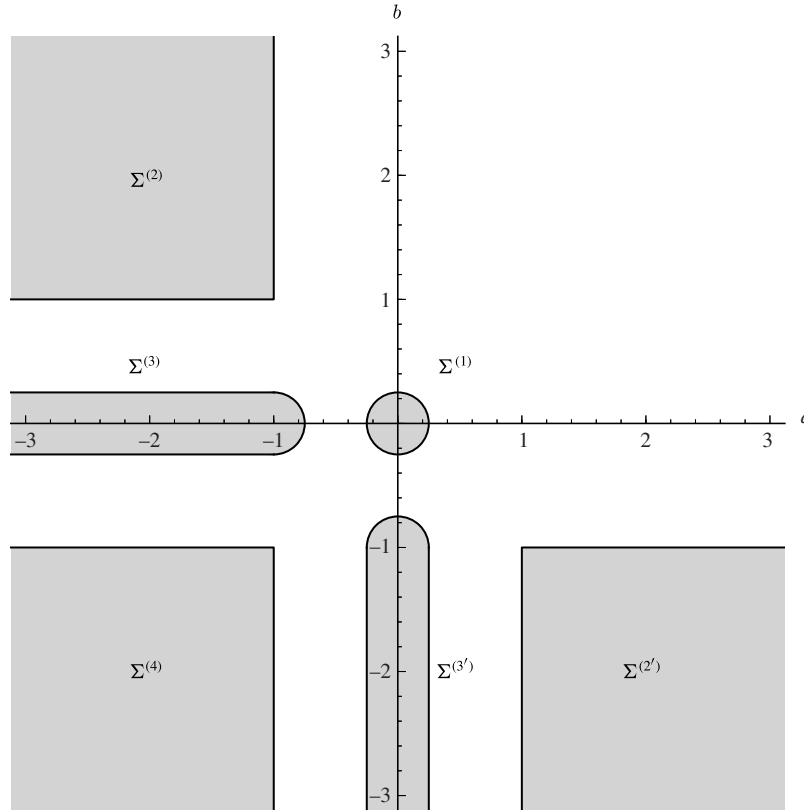
FIGURE 1. Infinity-types of Hecke characters of K .
