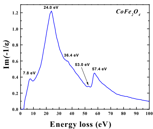
Figure 3. Energy Loss Function taken from cobalt ferrite
