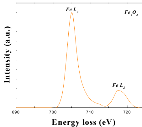
Figure 6. Fe L_{23} white lines taken from ferric oxide \text{Fe}_3\text{O}_4 .
