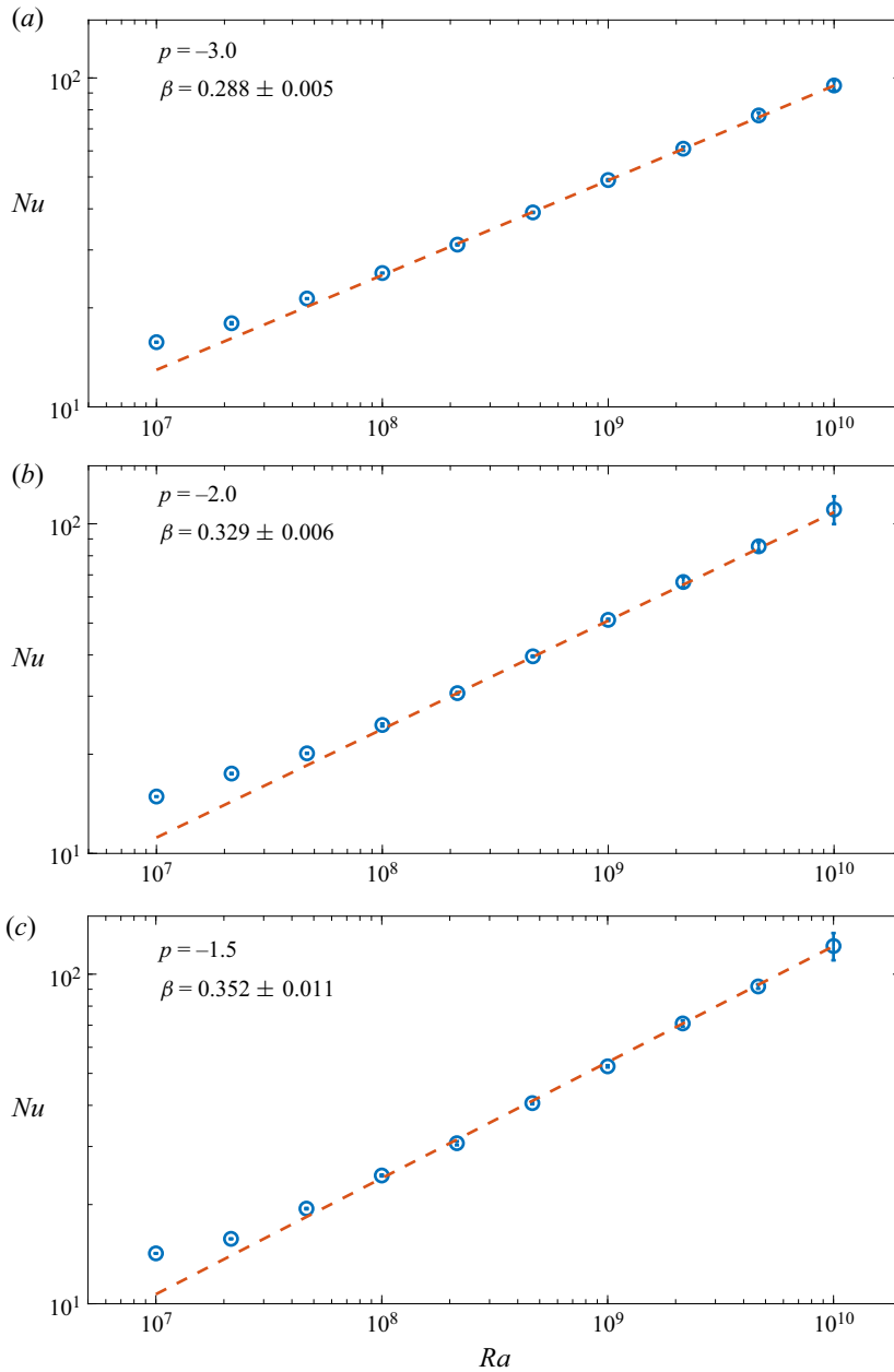
FIGURE 3. Plots of Nu(Ra) versus Ra \in [10^7, 10^{10}] for (a) p = -3.0 , (b) p = -2.0 and (c) p = -1.5 . Circles denote data from simulations and the dashed lines are the linear least-squares fits of \log Nu to \log Ra over the range Ra \in [10^8, 10^{10}] . The power laws are fit for the range Ra \in [10^8, 10^{10}] . For (a) p = -3.0 , Nu = 0.125 \times Ra^{0.288 \pm 0.005} ; (b) p = -2.0 , Nu = 0.055 \times Ra^{0.329 \pm 0.006} ; and (c) p = -1.5 , Nu = 0.037 \times Ra^{0.352 \pm 0.011} . The error bar on each Nu data point represents the standard deviation of the averaged Nu calculated from eight different horizontal sections, and the uncertainties in \beta are the 95 % confidence intervals.
