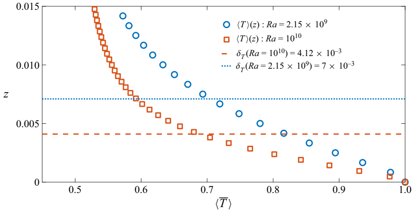
FIGURE 8. Horizontally and temporally averaged temperature profiles for Ra = 2.15 \times 10^9 (circles) and Ra = 10^{10} (squares) and p = -1.5 . The dotted and dashed lines show the boundary-layer thicknesses for Ra = 2.15 \times 10^9 and Ra = 10^{10} , respectively. There are 9 grid points in each boundary layer. The kinks at z = 0 are associated with the use of the mid-grid bounceback condition to impose no-slip and no-penetration boundary conditions in the lattice Boltzmann method. This version of the bounceback renders the effective wall to be between the first and second grid points (Succi 2001). Hence, the no-slip boundary condition effectively applies at a distance z = \Delta z/2 , where \Delta z is the grid size, above z = 0 where the temperature boundary condition is imposed. The calculation of Nu at the boundary takes this into account, and has been tested by reproducing the Nu(Ra) results from spectral simulations for flat boundaries (Toppaladoddi et al. 2015a).
