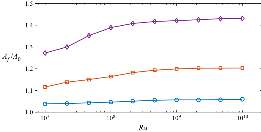
FIGURE 11. Ratio A_f/A_0 of effective transfer area to that of flat boundary as a function of Ra for different values of p : p = -3 (circles); p = -2 (squares); and p = -1.5 (diamonds).
