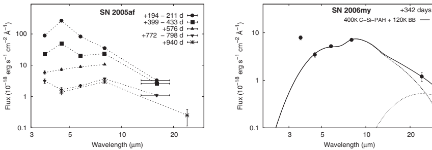
Figure 1. Left: Mid-IR SEDs of SN 2005af at different epochs. Right: An example of SED models: C-Si-PAH warm + cold BB components, SN 2006my (+342 days).
