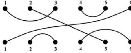
Figure 1. A Brauer algebra basis element for n = 6 .
