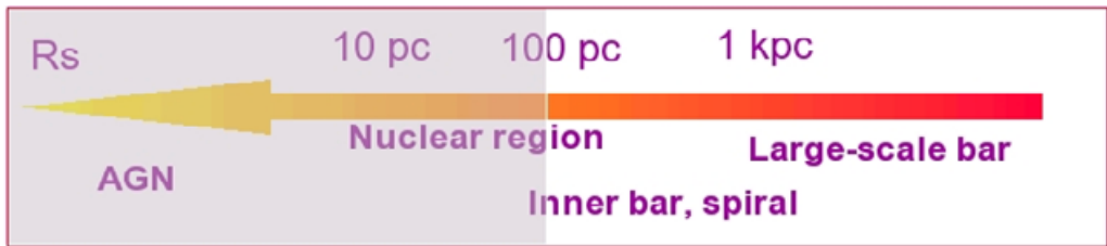
Figure 1. Sketch showing the wildly different scales we usually deal with when trying to link the nuclear activity with e.g. a large-scale bar. R_s is the Schwarzschild radius of the presumed black hole, \sim 10^{-5} pc for 10^8 M_\odot .
