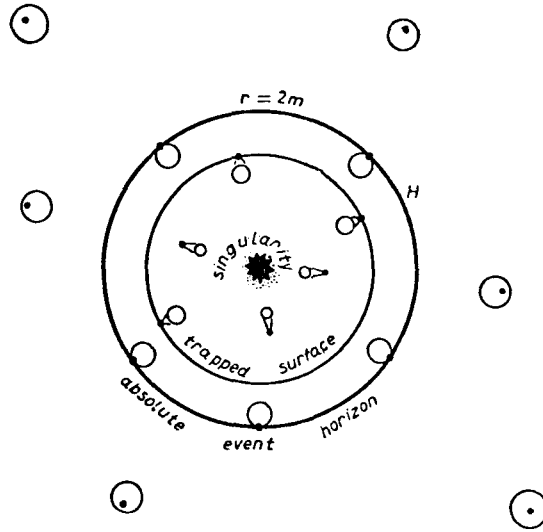
Figure 1. The spatial representation of the Schwarzschild black hole. The absolute event horizon occurs at the radius R_s = 2GM/c^2 . The wave fronts of light signals, emanating at various points at a slightly later time are shown. At large distances from the event horizon, the points lie at the centers of the respective wave fronts. At smaller distances, the wave fronts are displaced by the strong gravitational field present. The wave fronts emanating from points on the event horizon touch the event horizon on the inside and cannot emerge. Inside the event horizon the centers of emission are no longer even inside the wave fronts.
