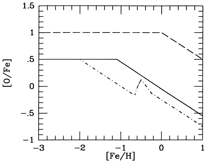
Figure 1. Schematic description of the [O/Fe] element ratio evolution as a function of [Fe/H] for three independent star-forming regions of differing massive-star IMFs and star formation rates.
