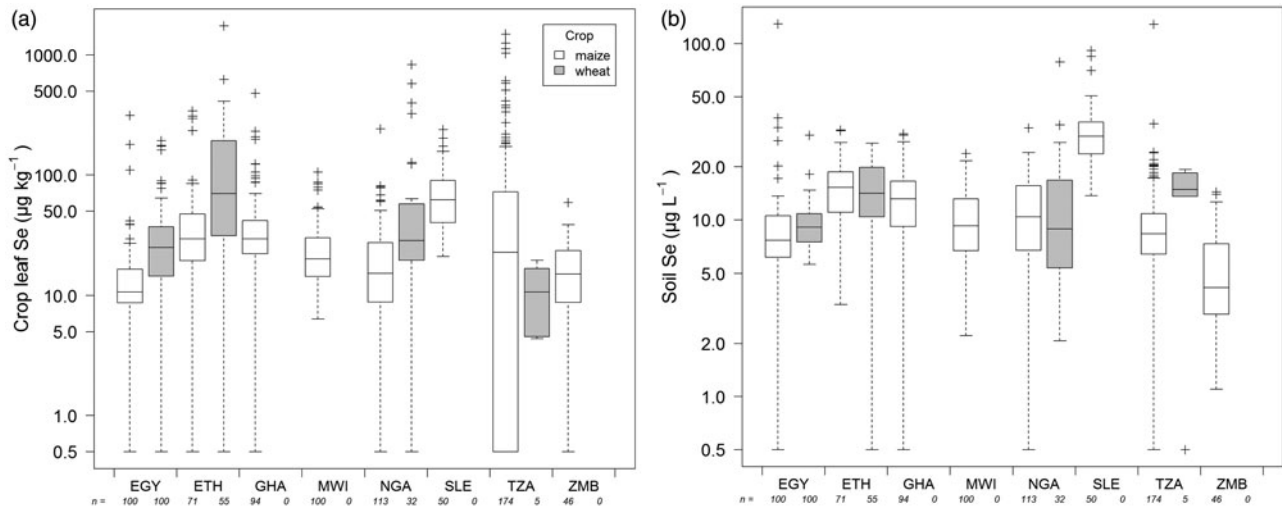
Fig. 4. Summary selenium (Se) concentration data from Sillanpää and Jansson (57) for (a) maize (white boxes) and wheat (grey boxes) leaves, (b) topsoil using acid ammonium acetate-EDTA universal extraction: Egypt (EGY), Ethiopia (ETH), Ghana (GHA), Malawi (MWI), Nigeria (NGA), Sierra Leone (SLE), Tanzania (TZA), Zambia (ZMB). Boxes represent upper and lower quartiles; whiskers are the 95 %-iles; medians are indicated within the boxes.
