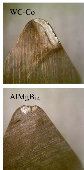
Fig. 2. Optical microscopy images of wear patterns on \text{AlMgB}_{14} and WC-Co cutting tools. The \text{AlMgB}_{14} presents catastrophic wear (fracture) while WC-Co presents crater wear. Crater wear is an indication of good wear.
