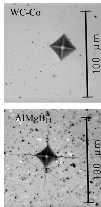
Fig. 3. Optical microscopy images of Vickers microhardness indents on an \text{AlMgB}_{14} cutting tool and on a WC-Co cutting tool. The \text{AlMgB}_{14} has a higher hardness (smaller indentation), and lower fracture toughness, as indicated by the longer cracks emanating from the corners of the Vickers indents.
