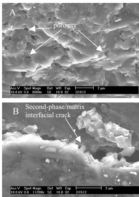
Fig. 1. Scanning electron microscopy images of two fracture surfaces of \text{AlMgB}_{14} cutting tools. A. Microporosity is present on the fracture surface. B. The crack interface between the second-phase particle and the matrix material is seen.
