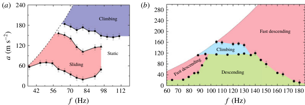
FIGURE 2. Phase diagram for a water drop (a) on a PMMA surface from (Sartori et al. 2015) and (b) on a LIS from Sartori et al. (2019). Note that the climbing region is reduced to a small patch on the LIS, whereas it is unbounded on the solid plate.
