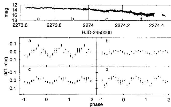
Fig. 2. Averaged spin profiles during the declining phase. The declining rate changed at HJD 2452274.0.
