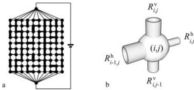
Fig. 1. (a) Random pipe or resistor network. (b) Close-up of a node and adjoining ducts.
