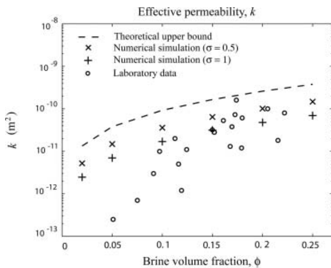
Fig. 2. Comparison of results for the two-dimensional network model with theoretical bounds and laboratory data. Laboratory data are from Freitag (1999) for young, artificially grown sea ice.
