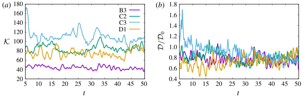
FIGURE 16. (Colour online) Time dependence of total kinetic energy density \mathcal{K} = (1/2)\langle |u|^2 \rangle_V (a) and scaled dissipation rate \mathcal{D}/\mathcal{D}_0 = \langle |\nabla u|^2 \rangle_V / Re^2 (b) for the various throttled simulations at large B whose fields are plotted in figure 3. Note that the dissipation fluctuates near, yet systematically below the target value \mathcal{D}_0 .
