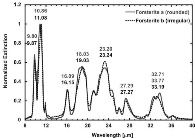
Figure 2: Normalized extinction vs. wavelength for two different shapes of forsterite particles. The grey solid line refers to the ‘Forsterite a’ (rounded), while the black dotted line refers to the ‘Forsterite b’ (irregular shapes).
