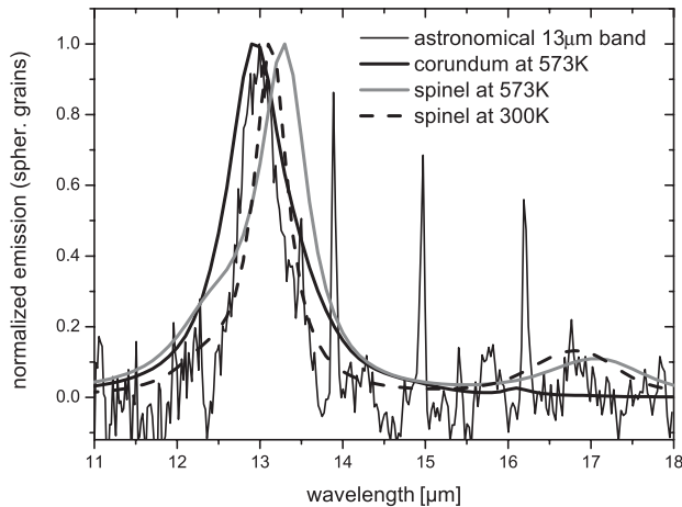
Figure 4: Comparison between the average profile of the astronomical 13\ \mu\text{m} emission band – as derived by Fabian et al. (2001) for a sample of oxygen-rich AGB stars – with the normalized emission spectra of corundum and spinel grains at temperatures of 300 K and 573 K.
