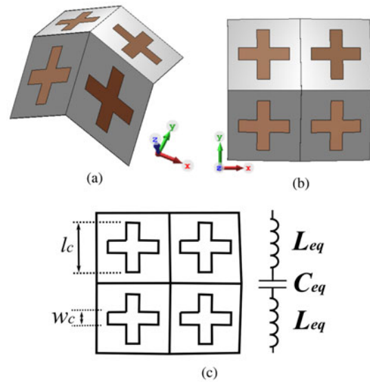
Fig. 3. Design of cross-dipole eggbox FSS element: (a) perspective view; (b) top view; and (c) equivalent circuit.
