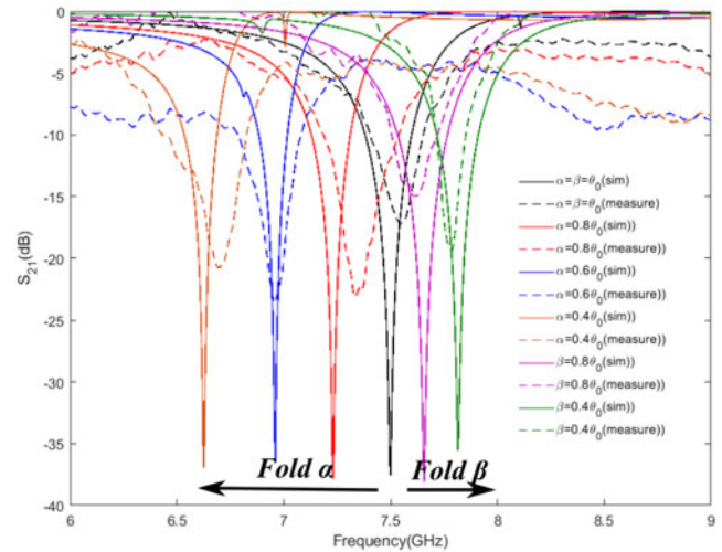
Fig. 8. Vertical ( y -axis) polarization with different folding angles simulation and measurement results.
