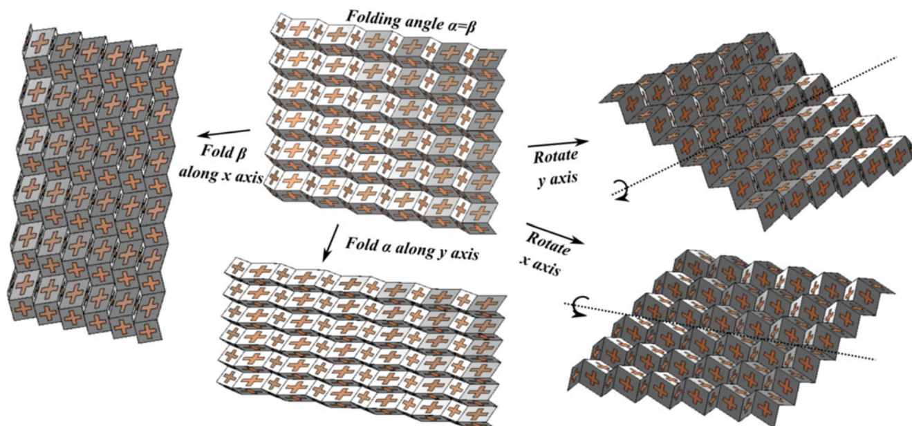
Fig. 4. Demonstration of 4-DOF tuning methodology: fold along x-axis; fold along y-axis; rotate x-axis; and rotate y-axis.
