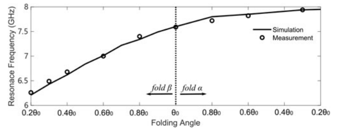
Fig. 9. Resonance frequency versus folding angles of horizontal polarization ( x -axis).
