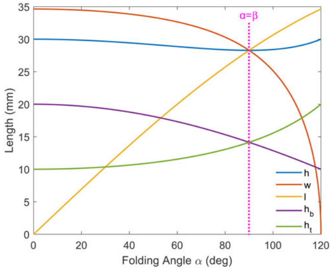
Fig. 2. Variation of different geometric parameters with folding angles \alpha from 0 to 120°.
