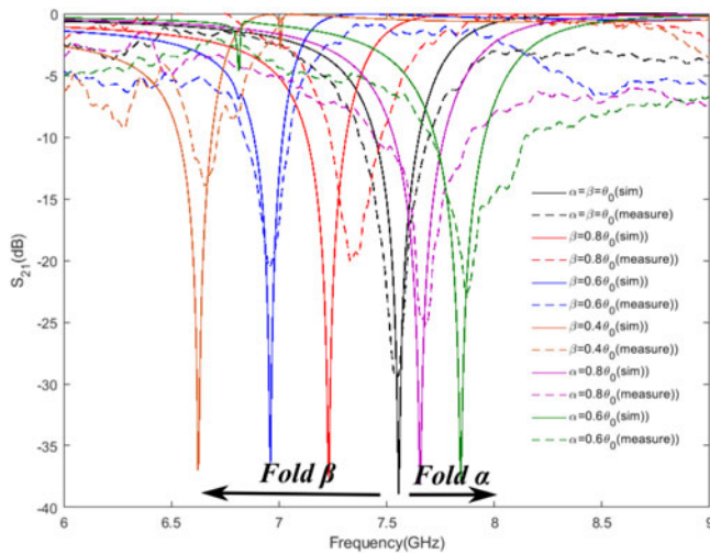
Fig. 7. Horizontal ( x -axis) polarization with different folding angles simulation and measurement results.
