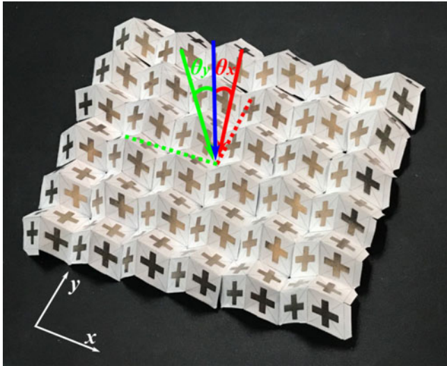
Fig. 6. Fabricated sample of 6 \times 6 cross-dipole eggbox FSS and incidence angles: normal incidence (blue), rotate y -axis (green), and rotate x -axis (red).
