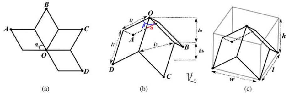
Fig. 1. Eggbox element design: (a) 2D flat eggbox outline pattern; (b) 3D-folded eggbox structure; and (c) 3D-folded eggbox volumetric boundary box.
