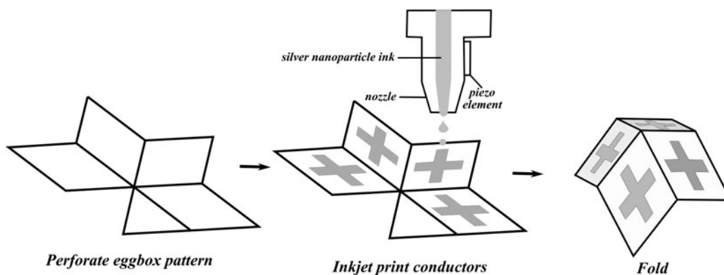
Fig. 5. Three-step fabrication process for eggbox FSS: perforate eggbox pattern; inkjet print conductive traces; and fold to 3D eggbox structure.
