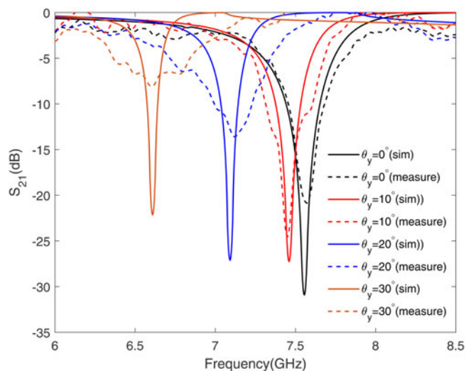
Fig. 10. Horizontal polarization ( x -axis) with different y -axis rotating angles simulation and measurement results.
