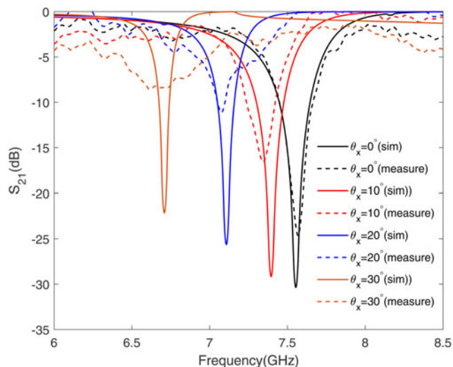
Fig. 11. Vertical polarization ( y -axis) with different x -axis rotating angles simulation and measurement results.
