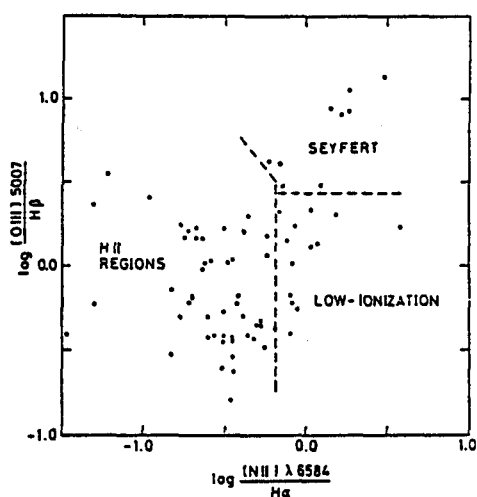
Fig. 5b: Observed line ratios in the spectra of interacting galaxies (Keel, 1985)
