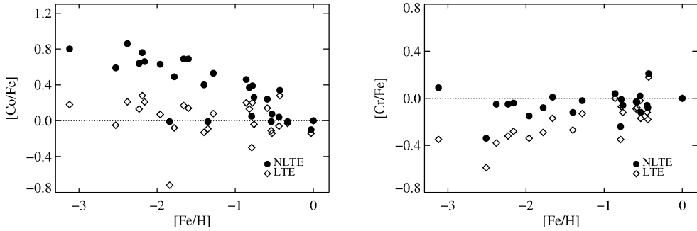
Figure 1. [\text{Co}/\text{Fe}] and [\text{Cr}/\text{Fe}] ratios in metal-poor stars as a function of metallicity. The abundances of Co and Cr are determined from the lines of neutral atoms.
