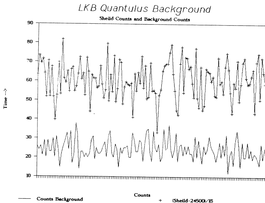
Fig 4. Count rate in the shield plotted with the background count rate in a glass vial for 10 days
