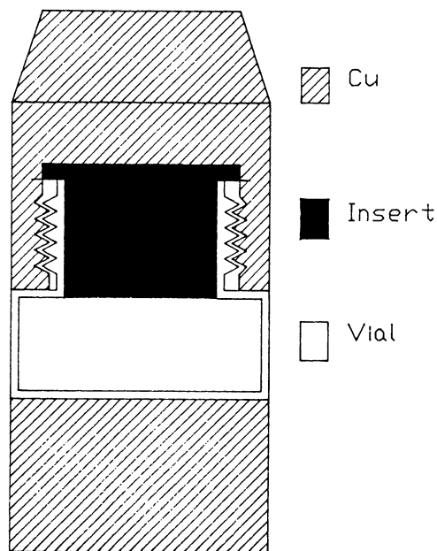
Fig 3. Cross-section of teflon vial with teflon insert
