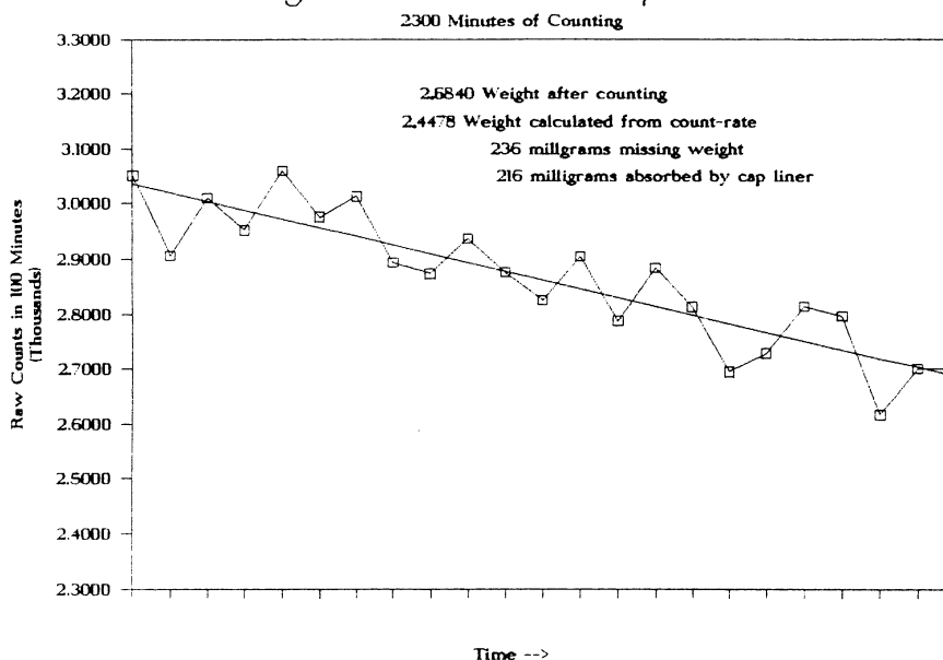
Fig 2. Best-fit line for a series of counts of an oxalic acid standard in a teflon vial
