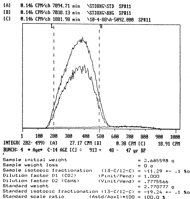
Fig 6. Age calculation output of sample A-5092 using the program supplied with the Quantulus as compared to the age calculated in our lab
