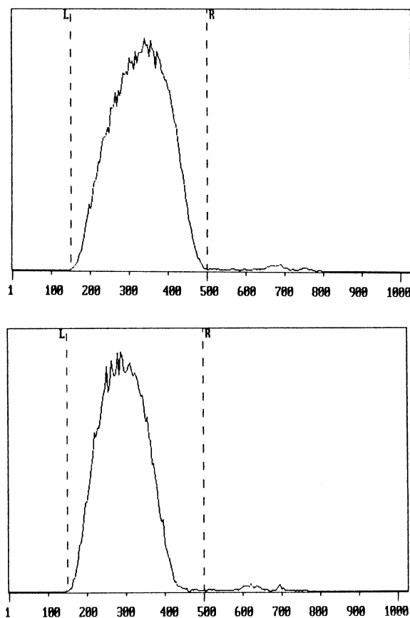
Fig 1. The same oxalic acid sample counted in two of the teflon vials supplied with the Quantulus
