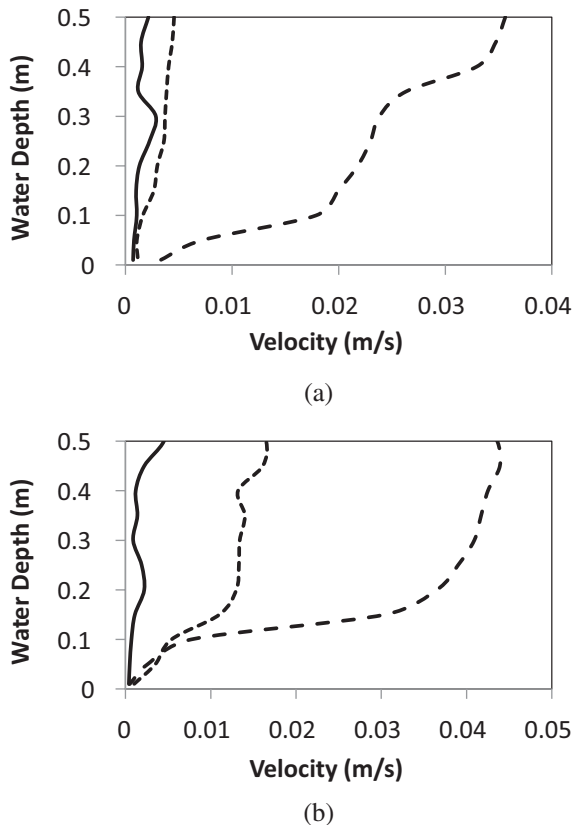
Fig. 8. Horizontal current velocity at different locations (N1: — N2: --- and N3: ·····) collected in summer 2008. (a) wind speed U_{10} of 3.13 \text{ m.s}^{-1} , direction of 308^\circ and (b) wind speed U_{10} of 4.83 \text{ m.s}^{-1} , direction of 275^\circ .
