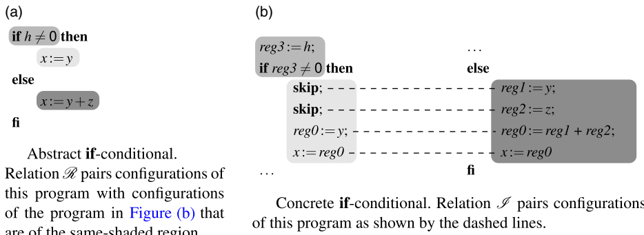
Fig. 2: Excerpts from a CVDNI-preserving refinement example with secret-dependent control flow: h contains a secret, y and z contain zero, and x is an untrusted sink. Reproduced from Sison & Murray (2019)—the example is originally from Murray et al. (2016b).
