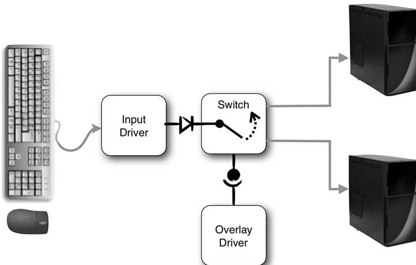
Fig. 6: Functional schematic of seL4 component architecture for CDDC HID switch. Reproduced from Murray et al. (2018).
