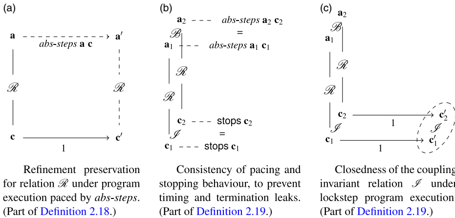
Fig. 4: Graphical depictions of decomposed refinement preservation obligations. Reproduced from Sison & Murray (2019).
