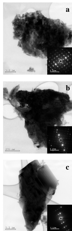
Fig. 2 TEM micrographs and diffraction patterns (inset) of 100-day used particles showing the presence of (a) (VO)_2P_2O_7 , (b) \beta - VOPO_4 and (c) \delta - VOPO_4 phases.
