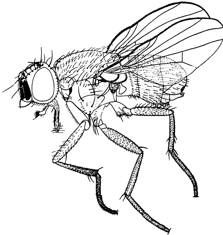
Atherigona varia (Meigen), ♂, from southern Europe (from Pont, 1973)
