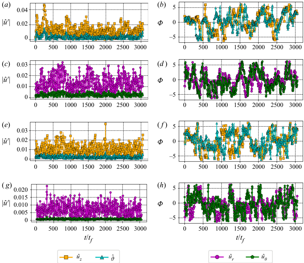
FIGURE 13. Temporal evolution of the scaled volume integrated Fourier coefficients of \hat{u}_z, \hat{v} (left pane) and \hat{u}_r, \hat{u}_\theta (right pane) for k = 5 (a–d), k = 10 (e–g) plotted by amplitude (left) and phase (right). The phase plots have been rescaled to cover a period of 4\pi to highlight the low frequency cycles that occur in the temporal evolution of these modes.
