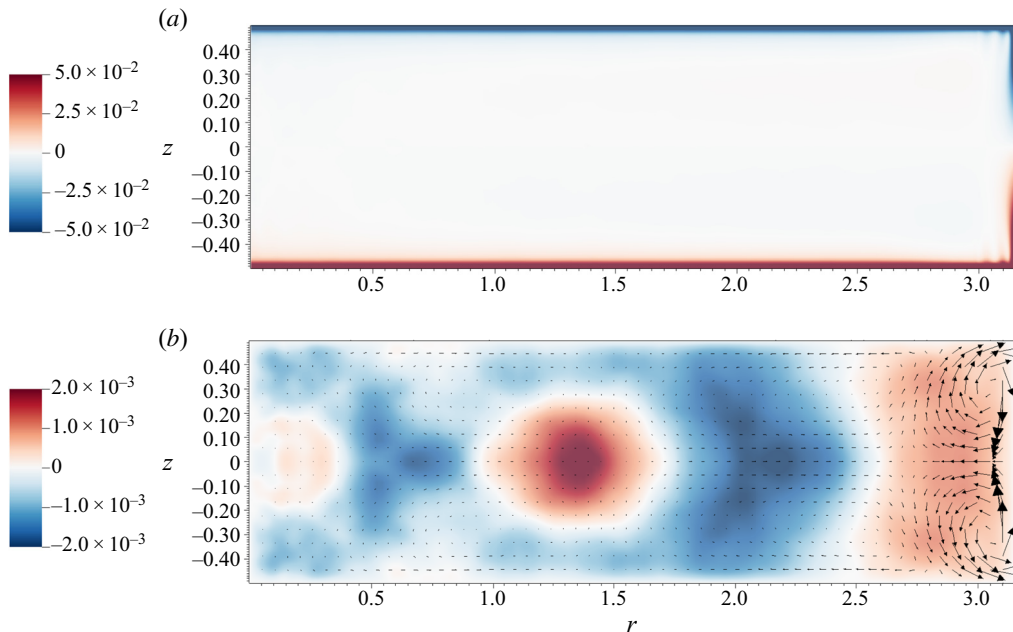
FIGURE 2. Azimuthal and temporally averaged mean fields. The colour plot in (a) corresponds to \langle \vartheta \rangle_{\theta,t} and in (b) it corresponds to \langle u_{\theta} \rangle_{\theta,t} , while the vector field in plot (b) is the two-dimensional vector of \langle \{u_r, u_z\} \rangle_{\theta,t} where the peak vector magnitude is 0.06 w_f . All length scales are normalized with H .
