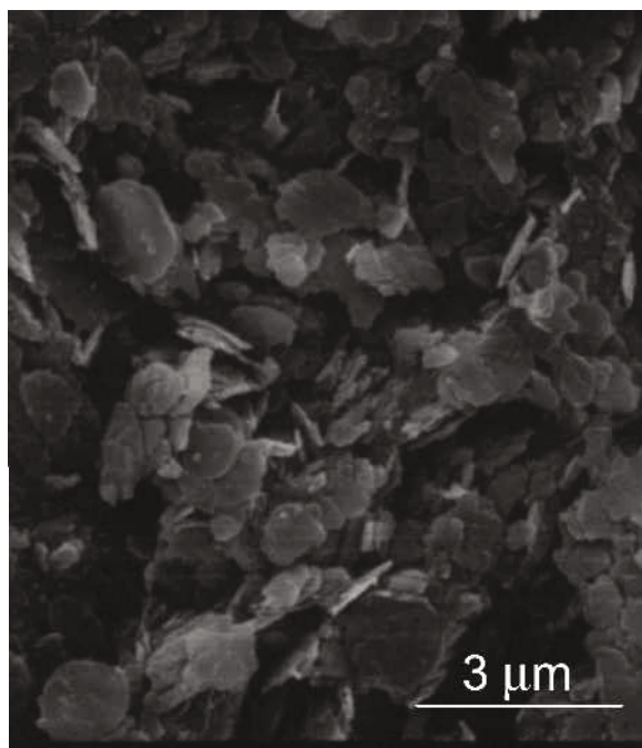
Figure 1. SEM image of lithiophorite.
