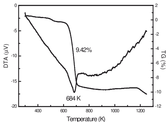
Figure 3. TG/DTA curves for lithiophorite.
