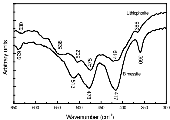
Figure 5. FIR spectra of lithiophorite and birnessite.
