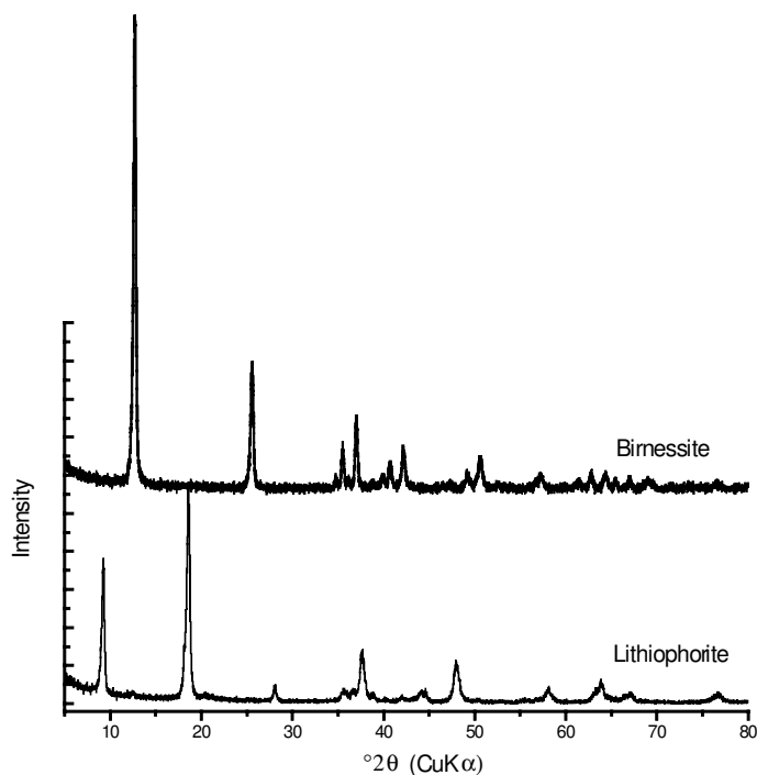
Figure 2. XRD patterns of birnessite and lithiophorite.
