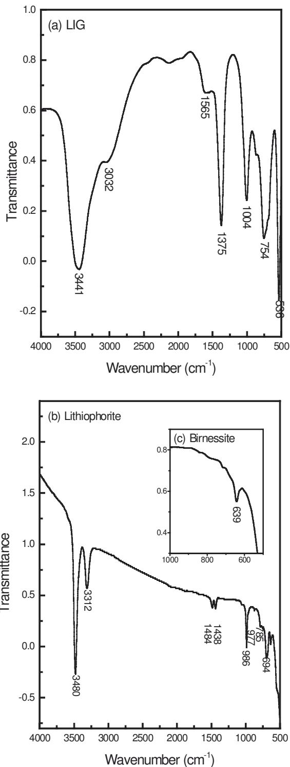
Figure 4. IR spectra of (a) Li-intercalated gibbsite (LIG), (b) lithiophorite. In the lower spectrum, the inset demonstrates the spectrum of (c) birnessite in the range 1000–500 \text{cm}^{-1} .
