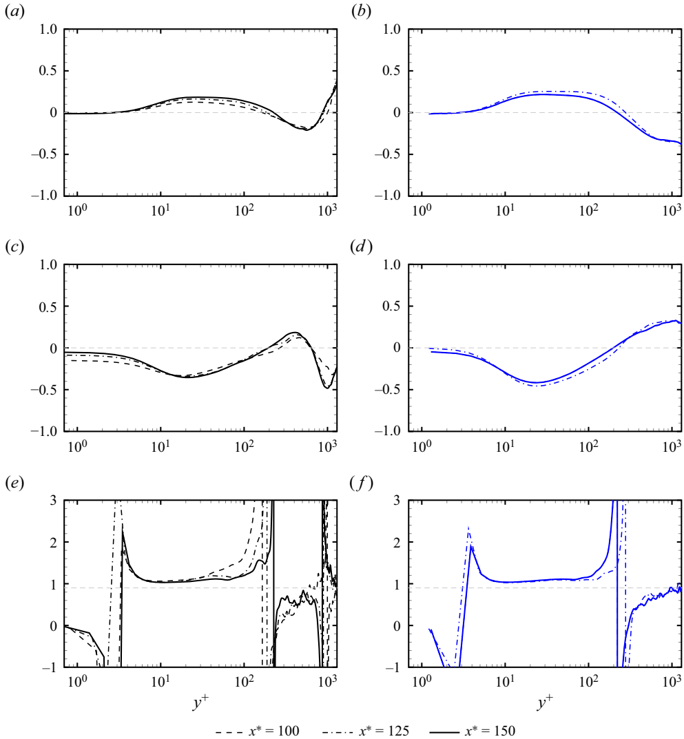
Figure 18. (a,b) Correlation coefficients between the fluctuations of wall-normal velocity and temperature R_{v'' , T''} . (c,d) Correlation coefficients between the fluctuations of streamwise velocity and temperature R_{u'' , T''} . (e,f) Turbulent Prandtl numbers Pr_t . (a,c,e) Reacting case (black). (b,d,e) Non-reacting case (blue). The axes R_{v'' , T''} = 0 and R_{u'' , T''} = 0 are superposed in (a–d) and Pr_t = 0.9 is superposed in (e,f).
