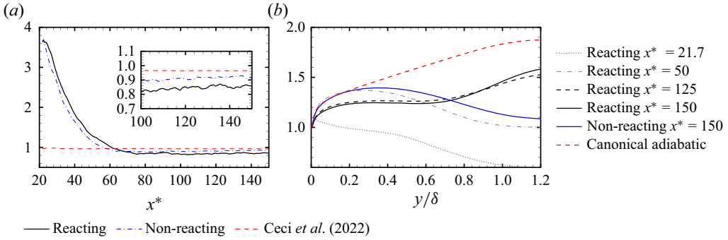
Figure 10. (a) Streamwise evolution of the peak value of Reynolds shear stress, \bar{\tau}_{t,xy}^{pk} , for both the reacting and non-reacting cases. A reference correlation from Ceci et al. (2022) is superposed. (b) Wall-normal profiles of local friction Reynolds number prefactor, \sqrt{\bar{\rho}/\bar{\rho}_w}(\bar{\mu}_w/\bar{\mu}) , at different streamwise positions, complemented by a canonical adiabatic model profile based on Pirozzoli & Bernardini (2011).
