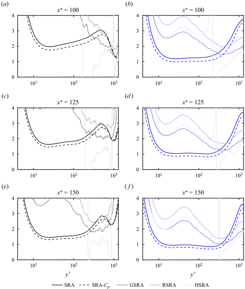
Figure 20. SRA and its extensions at different streamwise positions for the reacting (a,c,e) and non-reacting (b,d,f) cases. SRA and SRA- C_p represent the left-hand side of (5.4) and (5.5), respectively.
