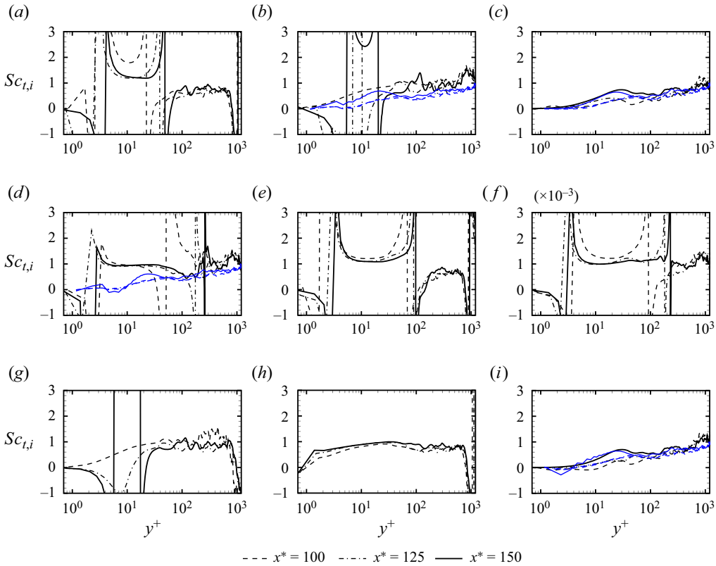
Figure 19. Turbulent Schmidt numbers Sc_{t,i} with inner scale y^+ : (a) O; (b) O_2 ; (c) H_2 ; (d) H_2O ; (e) OH; (f) H; (g) HO_2 ; (h) H_2O_2 ; (i) N_2 . The profiles are evaluated at three streamwise positions in the reacting (black) and non-reacting (blue) cases.
