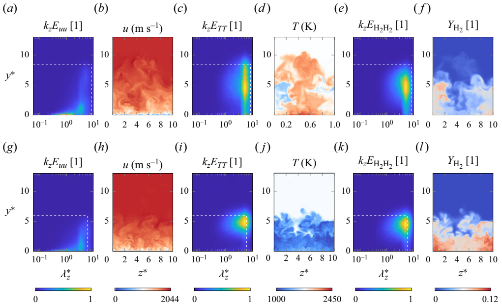
Figure 17. Premultiplied spectra k_z E_{uu} , k_z E_{TT} and k_z E_{Y_{H_2} Y_{H_2}} for reacting (a–f) and non-reacting (g–l) cases at x^* = 150 . The linear scale y^* is employed, and \lambda_z^* represents the wavelength corresponding to k_z under linear scale. The normalisation of E_{uu} and E_{TT} ensures their maximum value is unity. The white dashed lines indicate the boundary-layer thickness. Instantaneous streamwise sections of u , T and Y_{H_2} are provided using y^* and z^* as the wall-normal scale accordingly.
