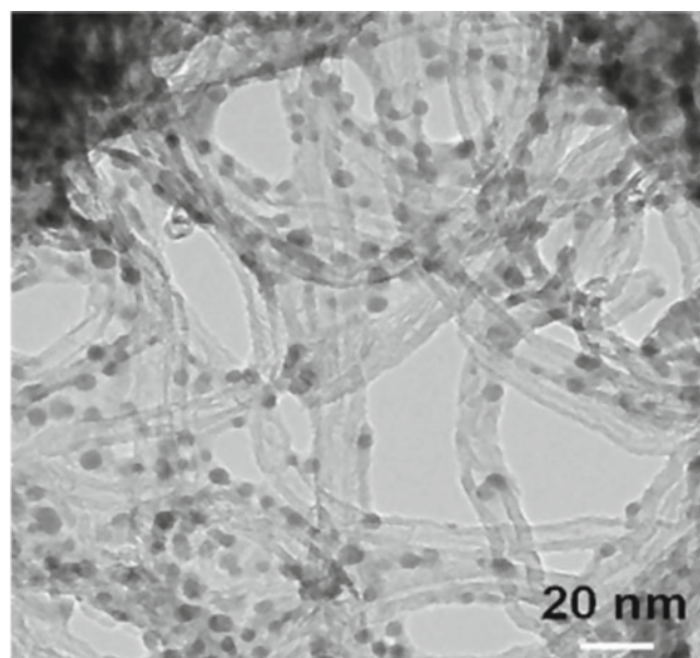
Fig. 5. TEM images of the nano hybrids PbS-QDs/MWCNTs showing coverage of PbS-QDs on the MWCNT surfaces.
