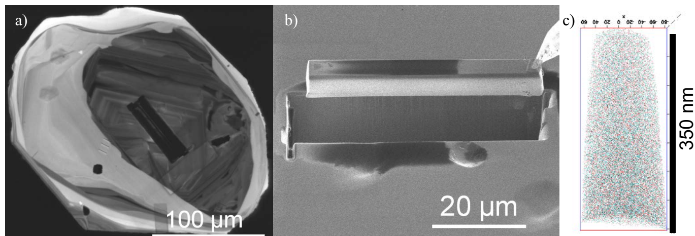
Figure 1. a) Cathodoluminescence image of the location of lift-out specimen (dark rectangle) seen on the polished section through the mid-section of zircon #1. Concentric banding results from mineral growth. b) Lift-out coupon in process, and c) an atom map from zircon #1 showing only Y in red and Pb in cyan. Note the uniformity of the Y and Pb distribution in this atom map with 4 \times 10^7 atoms.
