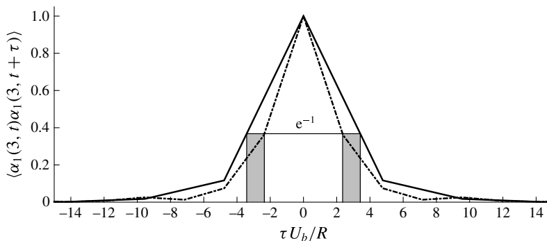
FIGURE 1. Autocorrelation of \alpha_{(m=1)}(m = 3, t) , revealing the temporal extent of \Phi_1(3; r) before a modal transition occurs: -\cdot-\cdot- , Re_D = 52\,000 ; — , Re_D = 104\,000 . Shaded area shows the convective length for which the correlations fall below e^{-1} , indicating the likely length of the meandering coherent structure.
