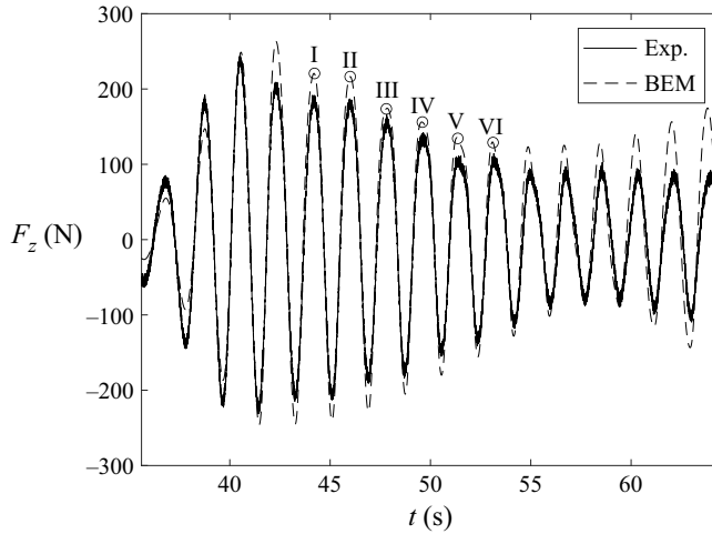
Figure 14. Vertical force F_z showing a decreasing trend when B = 30 cm, h = 60 cm, H/h = 0.1 , T = 1.8 s (solid line, experimental; dashed line, numerical).
