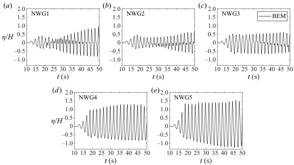
Figure 21. Free-surface elevation at five additional numerical WGs given in table 5 when B = 30 cm, h = 60 cm, H/h = 0.1 , \lambda = 1 , T = 1.8653 s.
