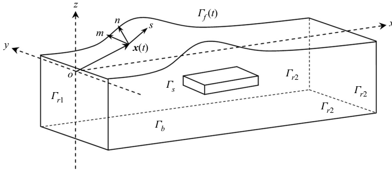
Figure 3. Sketch of the computational domain. The free surface \Gamma_f(t) is defined by the position vector \mathbf{x}(t) . Lateral boundaries are denoted by \Gamma_{r1} and \Gamma_{r2} , where \Gamma_{r1} is the boundary for the wavemaker and \Gamma_{r2} are other impermeable walls. The bottom and the structure are denoted by \Gamma_b and \Gamma_s , respectively. Tangential vectors at point \mathbf{x}(t) are defined as (\mathbf{s}, \mathbf{m}) and the outward normal vector as \mathbf{n} .
