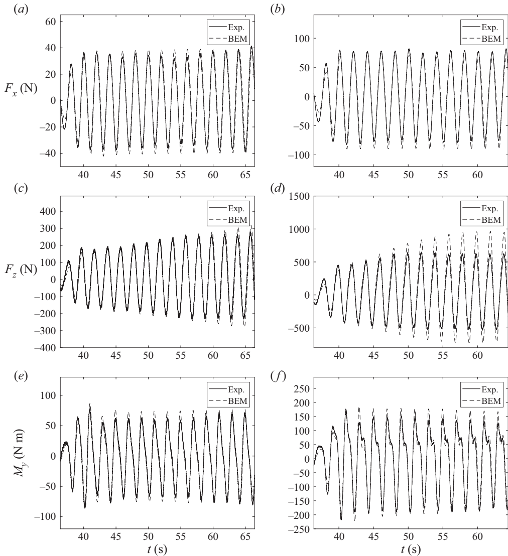
Figure 9. Same as figure 7 for T = 2 s.
