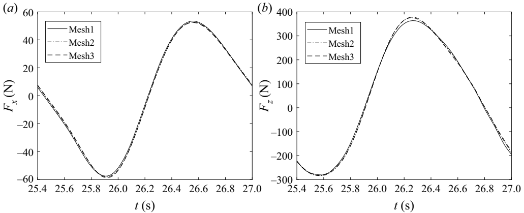
Figure 4. Comparison of the hydrodynamic load on the plate as a function of time t with three different mesh resolutions. (a) Horizontal force F_x ; (b) vertical force F_z .
