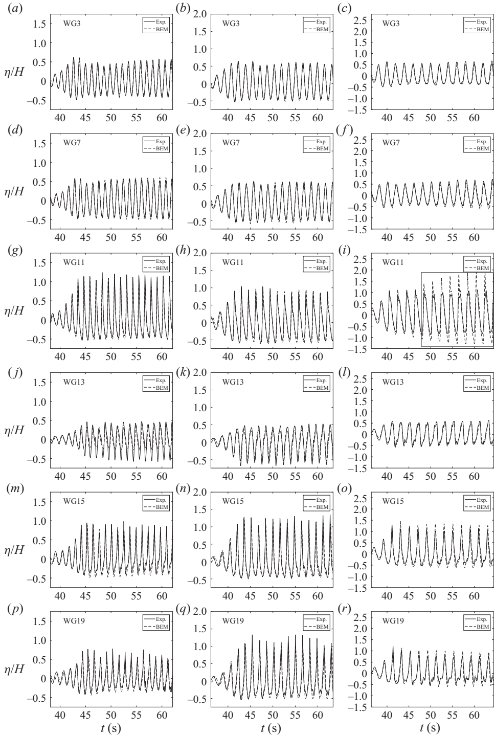
Figure 6. Same as figure 5 when B = 30 cm, h = 60 cm, H/h = 0.2 . The box on the third line and third column indicates the largest discrepancy between experiments and simulations.
