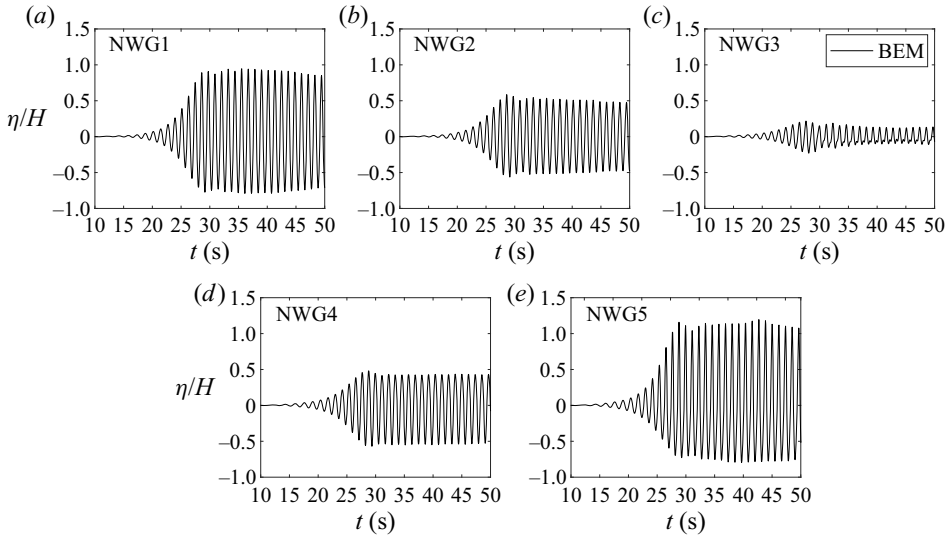
Figure 19. Free-surface elevation at five additional numerical WGs given in table 5 when B = 30 cm, h = 60 cm, H/h = 0.1 , \lambda = 1/2 , T = 1.1582 s.
