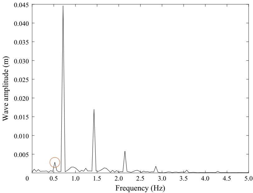
Figure 17. Fourier analysis of the wave elevation at WG11 when B = 30 cm, h = 60 cm, H/h = 0.1 and T = 1.6 s. The red circle indicates the frequency of the first sloshing mode.
