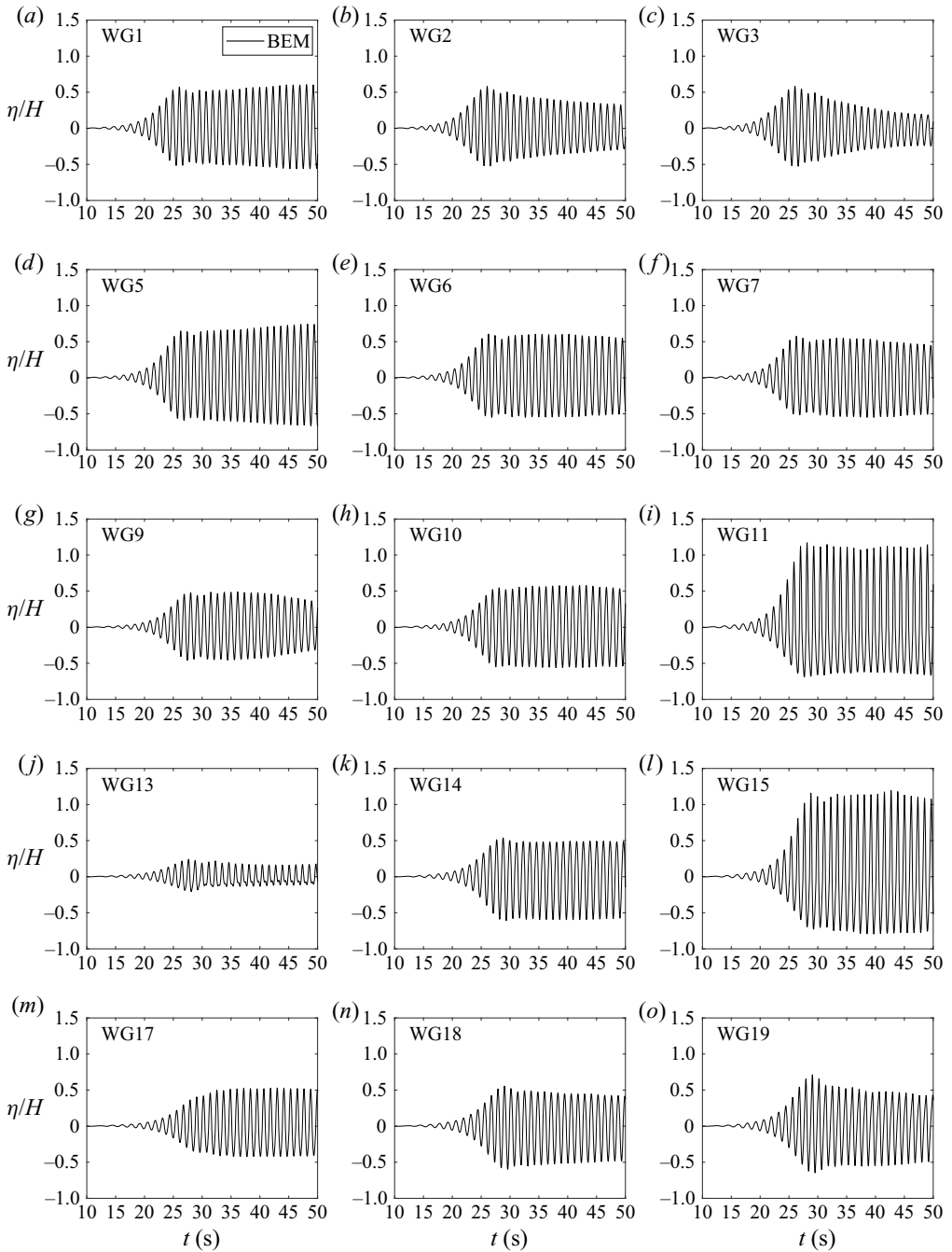
Figure 18. Free-surface elevation at 15 selected WGs when B = 30 cm, h = 60 cm, H/h = 0.1 , \lambda = 1/2 , T = 1.1582 s.
