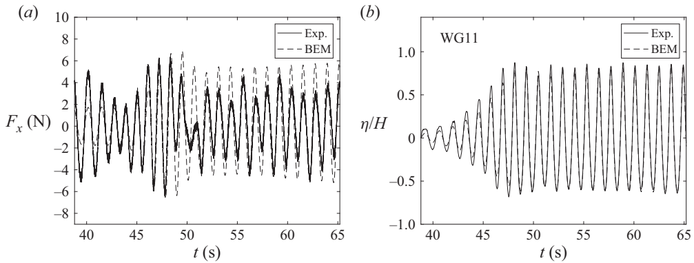
Figure 10. Horizontal force F_x and free-surface elevation at WG11 when B = 20 cm, h = 60 cm, H/h = 0.1 , T = 1.2 s (solid line, experimental; dashed line, numerical).
