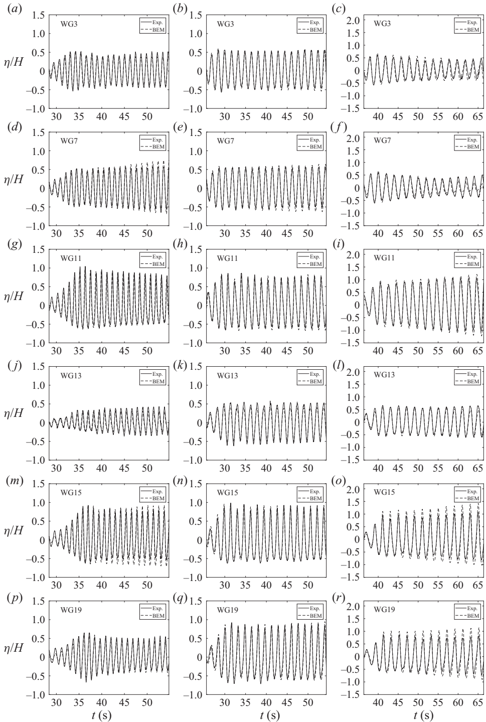
Figure 5. Comparison of the free-surface elevation at six selected WGs (WG3, 7, 11, 13, 15, 19) when B = 20 cm, h = 50 cm, H/h = 0.1 : T = 1.2 s (a,d,g,j,m,p); T = 1.6 s (b,e,h,k,n,q); T = 2 s (c,f,i,l,o,r). The solid and dashed lines represent the experimental and numerical results, respectively.
