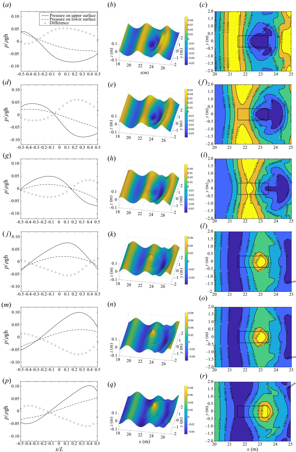
Figure 13. Sequence of numerical results illustrating the loading process. The parameters are B = 30 cm, h = 60 cm, H/h = 0.1 , T = 1.8 s. (a,d,g,j,m,p) Pressure distribution on the upper and lower faces of the plate and their difference; (b,e,h,k,n,q) snapshot of the free surface; (c,f,i,l,o,r) top view of the free surface. See figure 12 for the significance of the times A–F.
