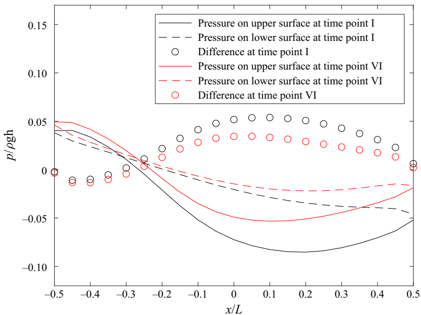
Figure 15. Numerically calculated pressure distribution at times corresponding to points I and VI (solid line, pressure distribution on the upper face of the plate; dashed line, pressure distribution on the lower face of the plate).
