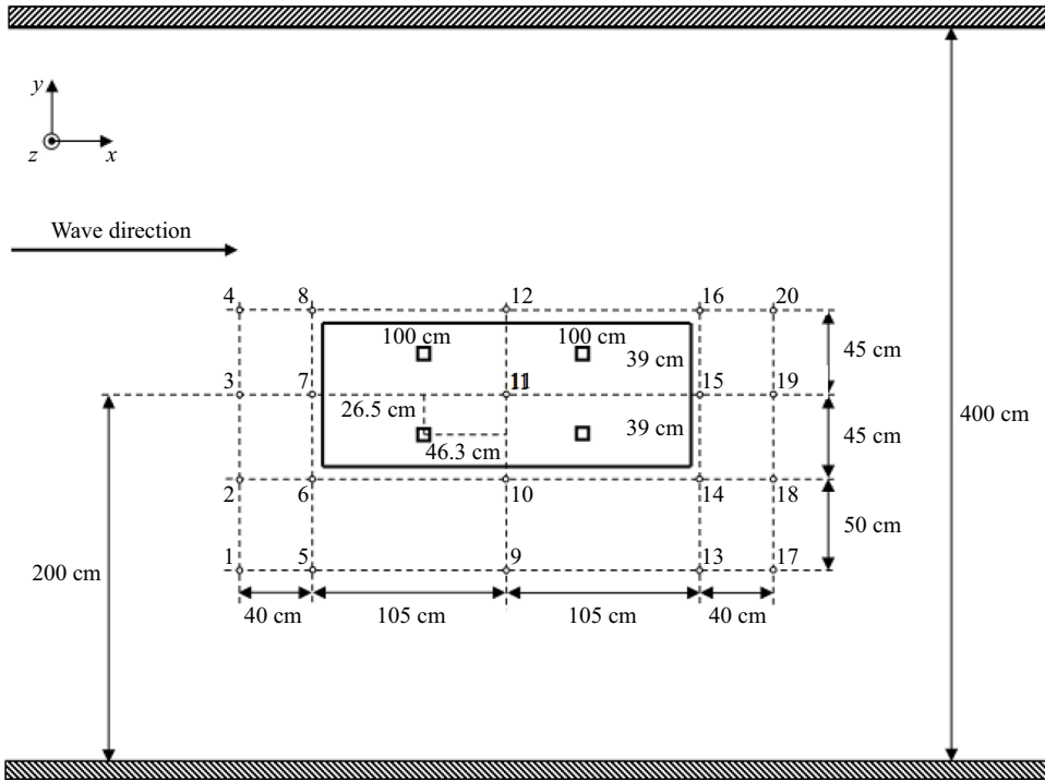
Figure 2. Top view of the wave flume and plate used for the laboratory experiments (all distances are in cm). The locations of the 20 WGs, labelled 1 to 20, are shown. They lie along four lines in the direction of the wave and five lines across the wave flume. The four squares indicate the locations of the four three-component force balance units.
