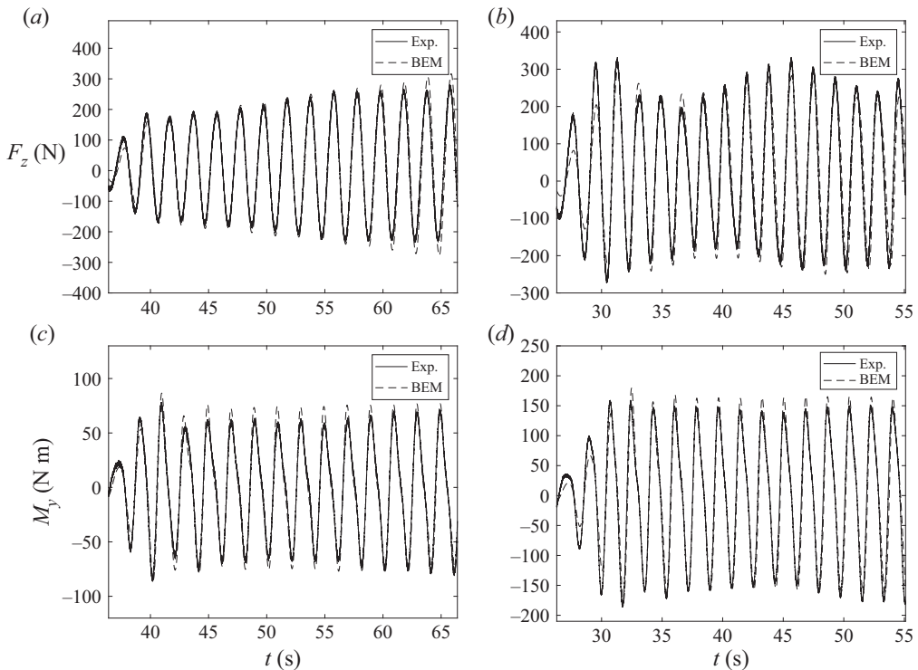
Figure 11. Vertical force F_z and moment M_y when B = 20 cm, h = 50 cm, H/h = 0.1 , T = 2 s (a,c) and B = 20 cm, h = 50 cm, H/h = 0.2 , T = 1.8 s (b,d) (solid line, experimental; dashed line, numerical).
