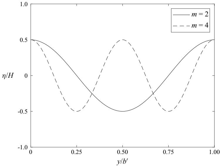
Figure 16. The first two even sloshing modes (solid line, m = 2 ; dashed line, m = 4 ).
