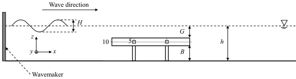
Figure 1. Side view of the wave flume and plate used for the laboratory experiments. The parameters that can be adjusted in the experiments are the wave height H , the water depth h , the distance from the bottom to the lower surface of the plate B and the depth of submergence of the plate G . The plate is 10 cm thick.
