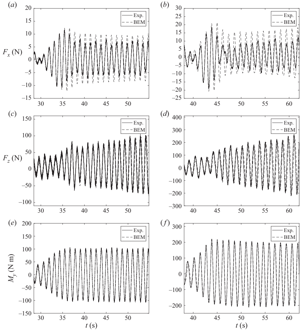
Figure 7. Horizontal force F_x (a,b), vertical force F_z (c,d) and moment M_y (e,f) when B = 20 cm, h = 50 cm, H/h = 0.1 (a,c,e) and B = 30 cm, h = 60 cm, H/h = 0.2 (b,d,f). Here T = 1.2 s (solid line, experimental; dashed line, numerical).
