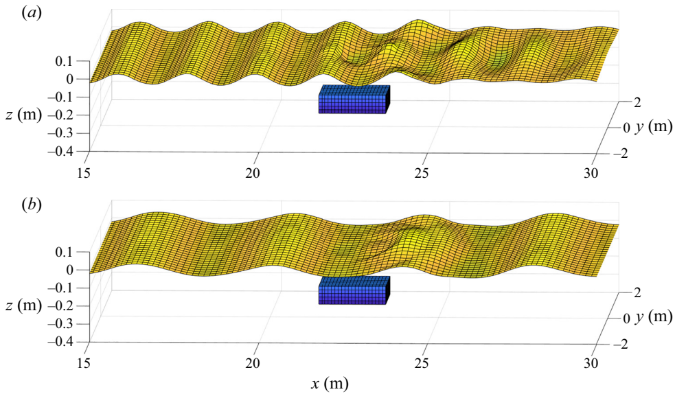
Figure 23. Snapshots of free surface when \lambda = 1/2 and \lambda = 1 .
