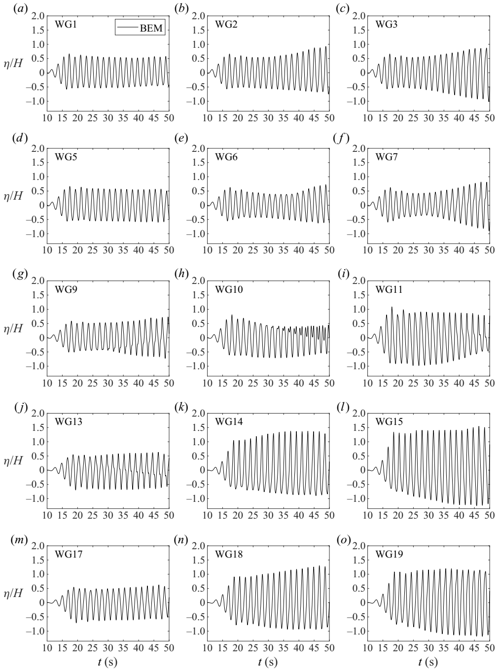
Figure 20. Free-surface elevation at 15 selected WGs when B = 30 cm, h = 60 cm, H/h = 0.1 , \lambda = 1 , T = 1.8653 s.
