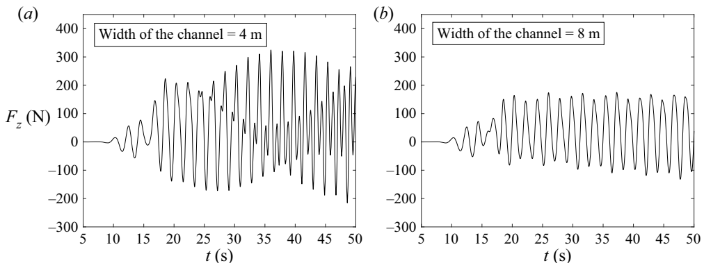
Figure 24. Vertical force exerted on the plate when the channel widths are equal to 4 m (a) and 8 m (b).
