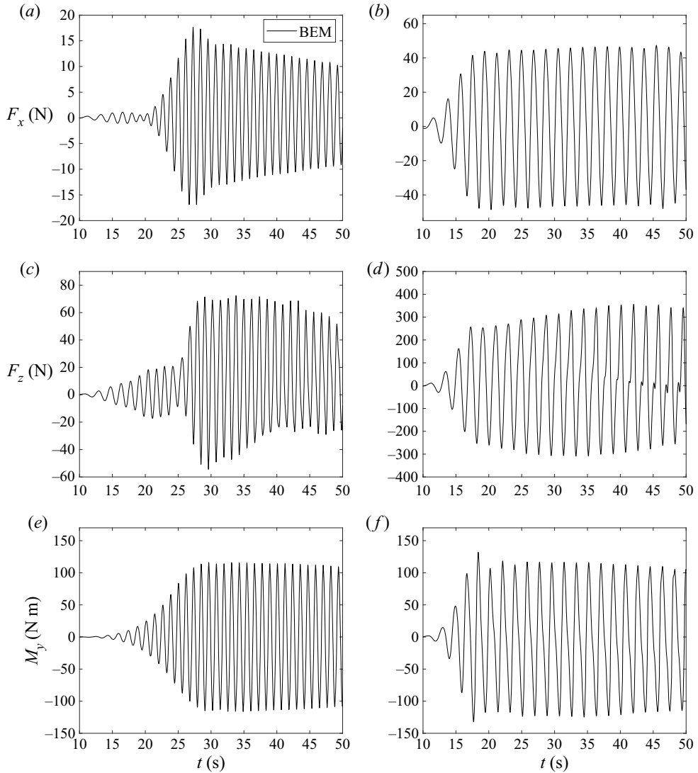
Figure 22. Horizontal force F_x , vertical force F_z and moment M_y when B = 30 cm, h = 60 cm, H/h = 0.1 : \lambda = 1/2 , T = 1.1582 s (a,c,e) and \lambda = 1 , T = 1.8653 s (b,d,f).
