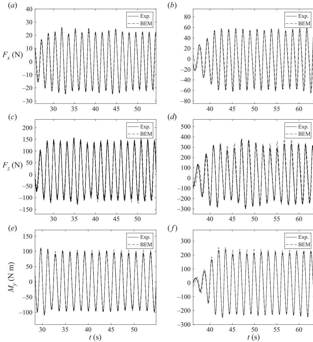
Figure 8. Same as figure 7 for T = 1.6 s.
