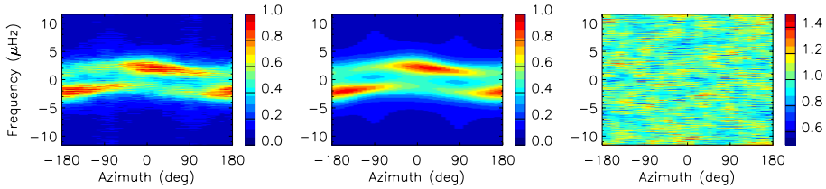
Figure 2. Same as previous figure but for latitude \lambda = -25^\circ . The fit returns the values \eta = 0.82 and \psi_{\max} = 29^\circ , i.e. the power is maximum in a direction that points 29^\circ equatorward of the prograde direction.
