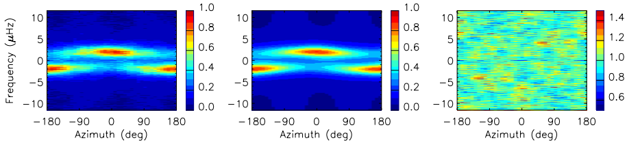
Figure 1. Power spectrum of the divergence signal for \lambda = 0 (equator) in 1997. The left panel shows a cylindrical section at constant wavenumber k = 115/R , as a function of azimuth, \psi , and frequency, \omega/2\pi . The middle panel is a fit to the data according to the model described in the text. In particular, \eta = 1.15 and \psi_{\max} = -2^\circ (excess power in the prograde direction). The right panel shows the ratio of the data to the fit.
