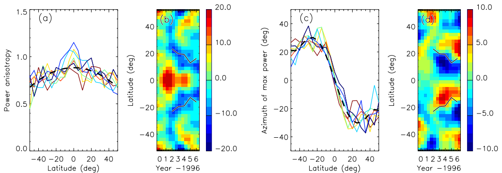
Figure 6. (a) Power anisotropy, \eta = 2A_1/A_0 , versus \lambda at k = 115/R . Each curve corresponds to a different year in 1996 to 2002). (b) Relative change of \eta with respect to the dashed line in panel (a), in percent. (c) Azimuth of maximum power, \psi_{\max} , versus \lambda at k = 115/R . (d) Residual \psi_{\max} after subtraction of the dashed line in panel (c). The scale bar has units of degrees.
