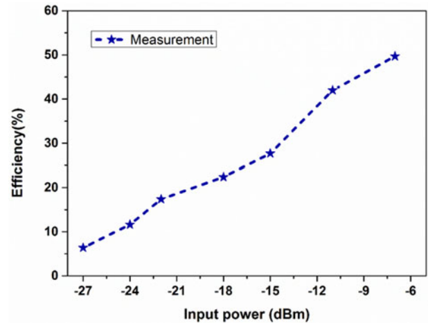
Figure 24. Measured result of conversion efficiency (input power to rectifier).
