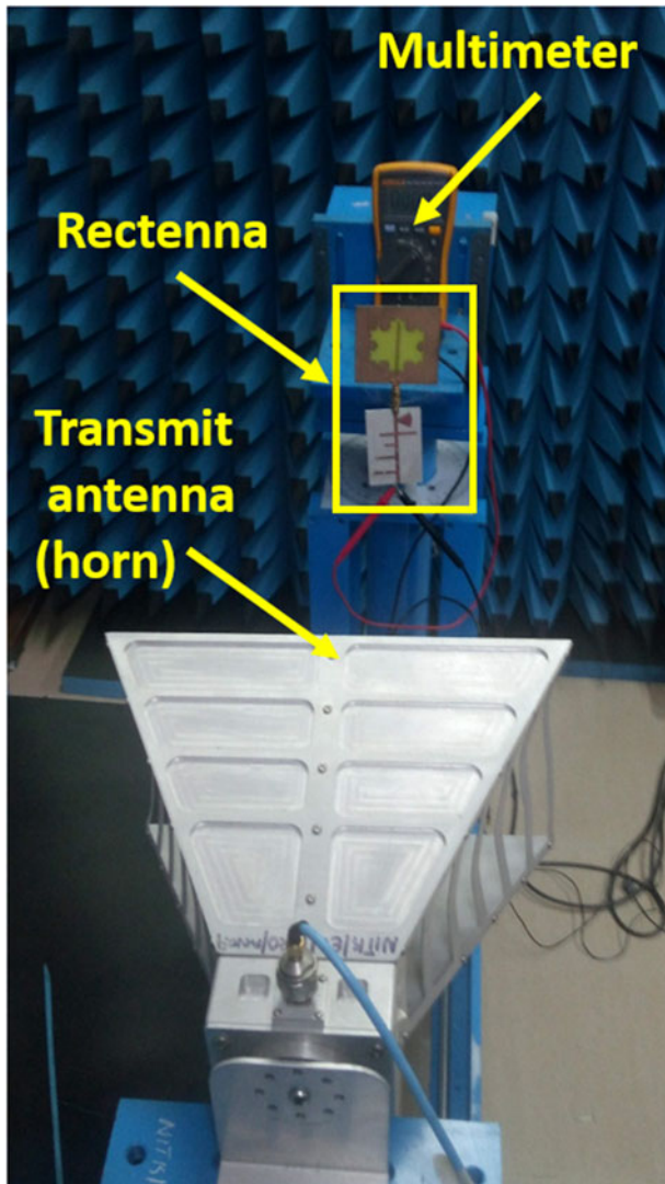
Figure 23. Measurement setup of rectenna in the anechoic chamber.
