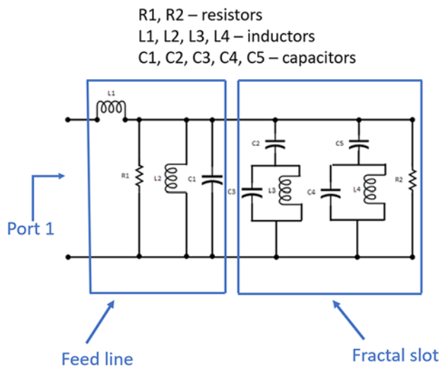
Figure 13. The proposed antenna equivalent circuit.
