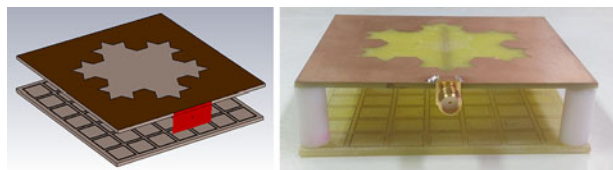
Figure 7. Computational and experimental configurations of the antenna with DRS reflector.
