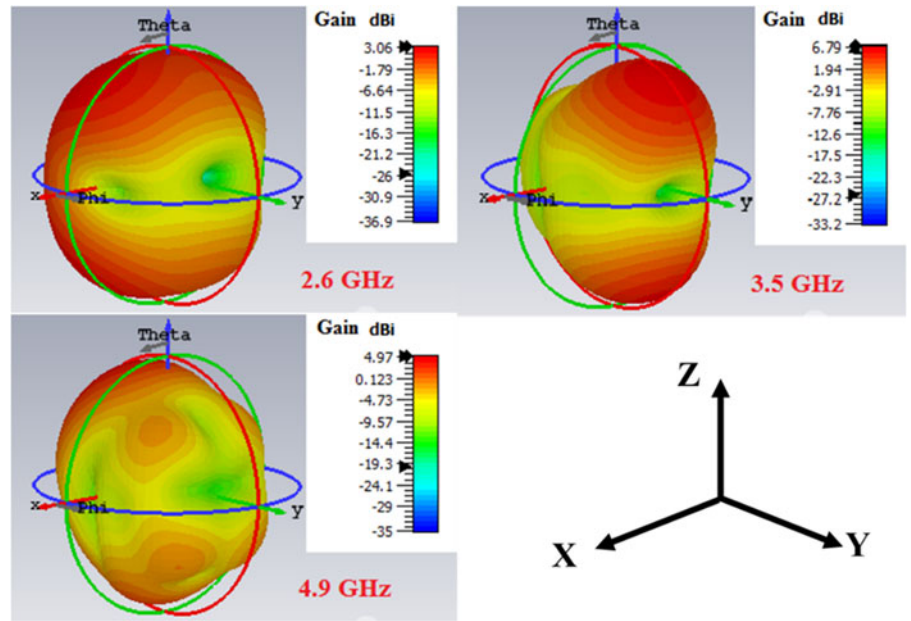
Figure 5. The computational results of the proposed antenna's three-dimensional radiation patterns without a reflector.
