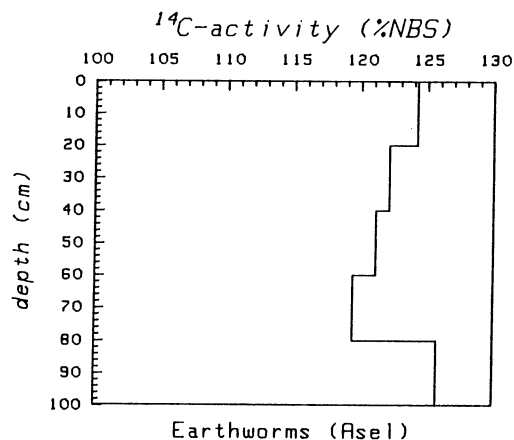
Fig 8. ^{14}\text{C} activity of earthworms at different depths of the Asel profile
