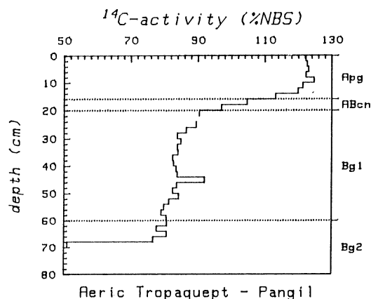
Fig 5. ^{14}\text{C} activity depth distribution of the Pangil profile
