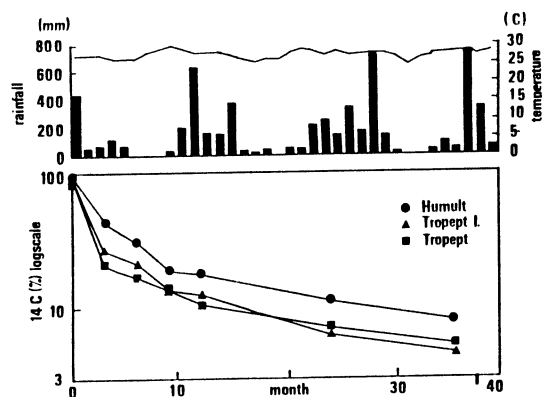
Fig 3A. Decomposition of organic matter in terrestrial soils of the Philippines
