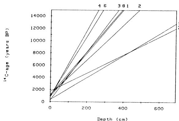
Fig 4. Mollisol dates; regression lines represent countries of origin (1 FRG, 2 CSSR, 3 USSR, 4 Hungary, 5 Australia, 6 Bulgaria, 7 Tunisia – surface, 8 Tunisia – covered)
