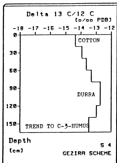
Fig 7. \delta^{13}\text{C} profile curve of a Sudanese Vertisol
