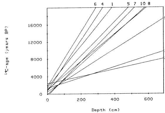
Fig 6. Vertisol dates; regression lines represent countries of origin (1 FRG, 2 Sudan, 3 Tunisia, 4 Argentina, 5 Israel, 6 Bulgaria, 7 Italy, 8 Spain, 9 Portugal, 10 Australia)
