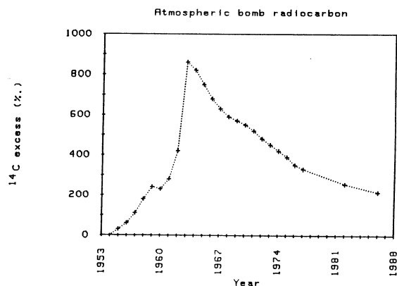
Fig 2. Atmospheric bomb C level (after Tans, 1981; continued by our measurements)
