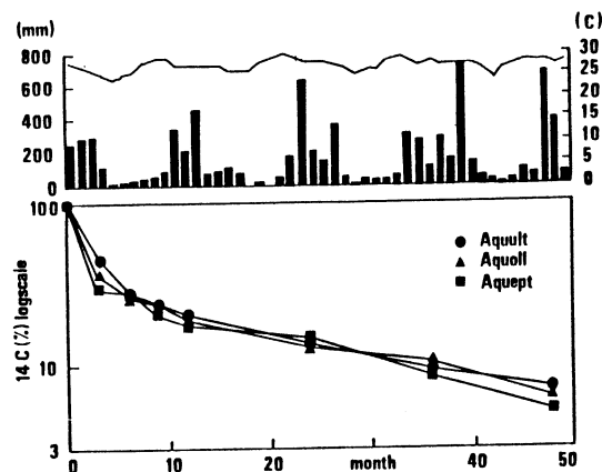
Fig 3B. Decomposition of organic matter in submerged soils of the Philippines
