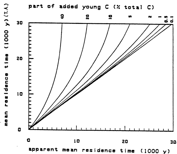
Fig 1. Effect of admixture of modern carbon on ^{14}\text{C} age
