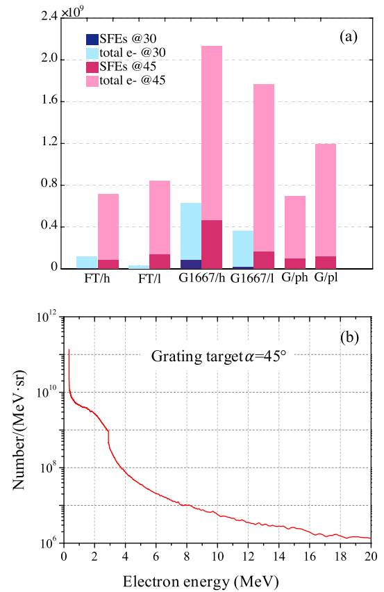
Figure 4. In the chart (a), the total numbers of electrons ( \phi = 0^\circ\text{--}180^\circ ) including the SFEs ( \phi = 0^\circ\text{--}10^\circ ) with energies larger than 1.5 MeV using GT ( \lambda_g = 1667 \text{ nm} ) and FT at \alpha = 30^\circ (blue colors) and \alpha = 45^\circ (magenta colors) for different interaction conditions are shown. Abbreviations ‘l’ and ‘h’ stand for low- and high-contrast conditions, respectively, while ‘p’ stands for the case when the grating’s grooves were parallel with the incident laser plane. In all other cases discussed before, the grooves were orientated perpendicularly to the incidence plane. (b) A typical electron energy spectrum of the fast electrons recorded at the high-contrast conditions at \phi = 3^\circ from the GT tangent direction ( \lambda_g = 1667 \text{ nm} ) and for \alpha = 45^\circ .
