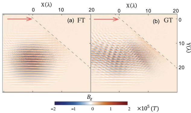
Figure 5. Snapshots of 2D PIC simulations showing the magnetic field components B_z at t = 28 \cdot T_L for the two targets: FT in (a) and GT ( \lambda_g = 2\lambda_L ) in (b). Laser is incident at \alpha = 45^\circ and its direction is marked by the red arrow. The initial target surface position is indicated by the dotted line and a preplasma of scale length L_n = 60 nm was modeled at the front of the target.
