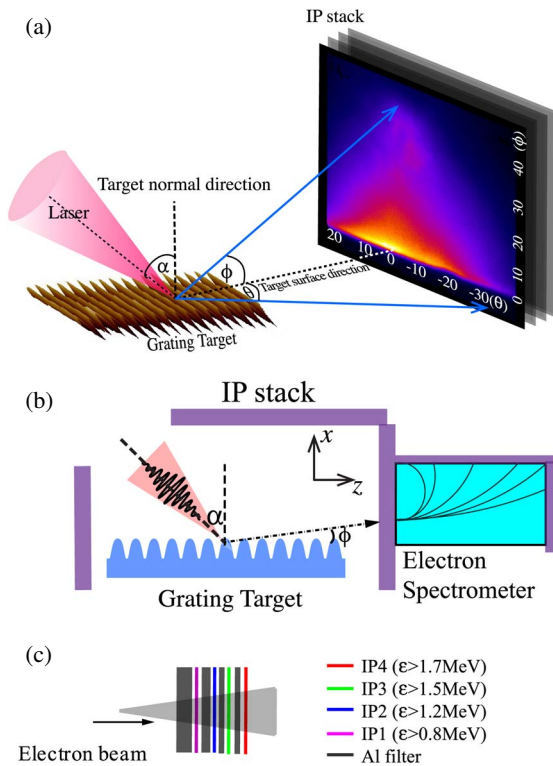
Figure 1. (a) A schematic of the experimental setup showing the interaction geometry. A laser pulse is focused at an incident angle of \alpha onto a GT with a periodical modulation of \lambda_g = 1667 nm and of vertical amplitude h_g = 80 nm. The spatial distribution of surface electrons is recorded by image plate (IP) stacks. \phi and \theta are the azimuthal and polar angles, respectively, used to describe spatially the electrons. (b) The side-on view of experimental setup. Three IP stacks (shown in purple color) are arranged around the interaction point to detect the high energy electrons emitted within an angular range of \phi between 0^\circ and 180^\circ , and an electron spectrometer is oriented along the target surface direction to measure the energy spectra of the surface fast electrons. (c) The IP stack consists of IPs and aluminum filters of different thicknesses, allowing the electron spatial distribution for different energies to be obtained.
