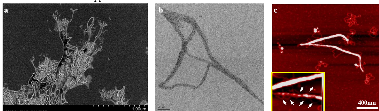
Figure 1. Microscopic images of complexation of plasmid DNA and RNT: (a) SEM, (b) TEM, (c) AFM. An inset shows the plasmid DNAs wrap the RNT periodically as indicated by arrows.
