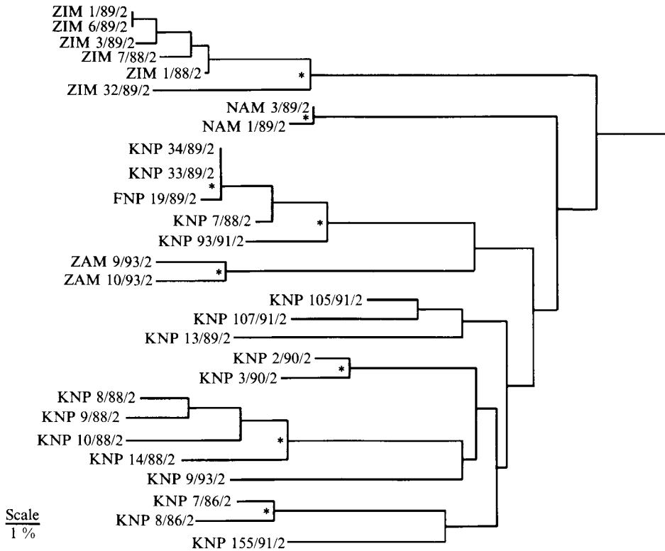
Fig. 6. Dendrogram depicting the relationships between the SAT-2 buffalo isolates from southern Africa between 1986 and 1993. The percentage sequence divergence between any two strains is the sum of the distances along the abscissas to the connecting node. *, Significant nodes.
