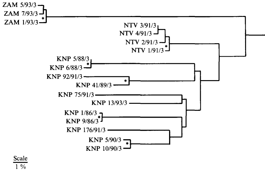
Fig. 8. Dendrogram depicting the relationships between the SAT-3 buffalo isolates from southern Africa between 1986 and 1993. The percentage sequence divergence between any two strains is the sum of the distances along the abscissas to the connecting node. *, significant nodes.
