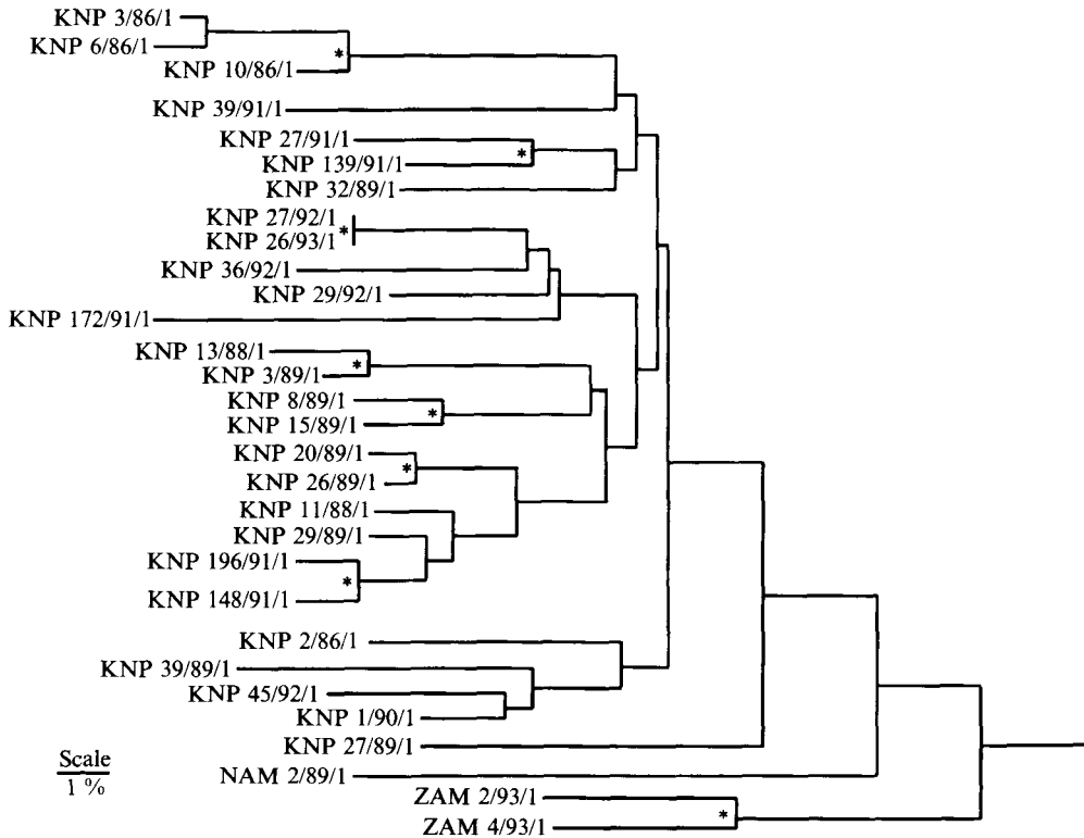
Fig. 4. Dendrogram depicting the relationships between the SAT-1 buffalo isolates from southern Africa between 1986 and 1993. The percentage sequence divergence between any two strains is the sum of the distances along the abscissas to the connecting node. *, Significant nodes.
