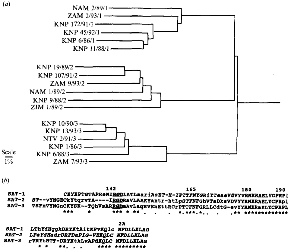
Fig. 2a. Dendrogram depicting the relationships between selected SAT-1, 2 and 3 buffalo isolates from southern Africa. The percentage nucleotide sequence divergence between any two strains is the sum of the distances along the abscissas to the connecting node. The last number in the virus designation indicates the SAT type. Fig. 2b. Alignment of the consensus amino acid sequences of SAT-1, 2 and 3. Upper case indicates consensus between all the sequences of a serotype, while lower case indicates that some variation occurred. *, Homology between all three consensus sequences; ., conservative change; —, gaps to accommodate alignment; RGD , cell attachment motif.
