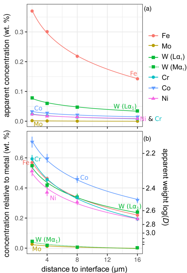
Fig. 6. Simulations along a transect from a forsterite–metal ( \text{Fe}_{15}\text{CrCoNiMoW} ) interface [Exp4], showing points in the forsterite side only. Uncertainties and curves as in Figure 4. Dotted line shows \text{W}\text{M}\alpha_1 as an alternative to \text{W}\text{L}\alpha_1 ; in (a) it is identical to the curve for Mo and thus is not visible. a: Apparent concentrations in the forsterite, as a function of distance from the interface with the metal. b: Concentrations of the elements divided by their concentrations in a simulated metal \text{Fe}_{15}\text{CrCoNiMoW} standard. Because the trace elements do not have equal weight concentrations in the metal, the fluoresced concentrations are also shown as percentages of the concentration in the metal.
