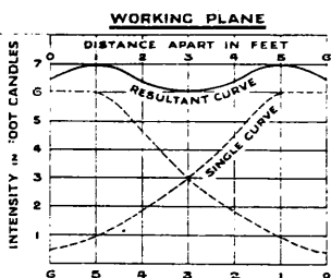
REPRESENTATIVE ILLUMINATION CURVE ON WORKING PLANE FOR INTENSIVE TYPE REFLECTOR NO. E. 6333 SPACED 6 FEET APART USING 60 WATT M.F. LAMPS
