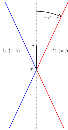
FIGURE 7. The cones C_+(x, \beta) and C_-(x, \beta) .
