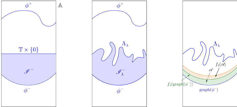
FIGURE 9. Here, \mathcal{S}^- := \text{int}(C^-) is the part of the instability region \mathcal{S} = \text{int}(C) that lies below the zero section \mathbb{T} \times \{0\} , while \mathcal{S}_\lambda^- := \text{int}(C_\lambda^-) is the connected component of \mathcal{S} \setminus \Lambda_\lambda bounded by \Gamma_{\phi^-} .
