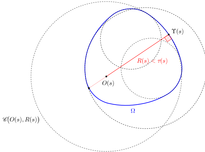
FIGURE 3. The geometric condition \max_{s \in \mathbb{T}} \tau(s)\mathcal{K}(s) < -1 in Definition D. Here, R(s) := -1/\mathcal{K}(s) is the radius of curvature, and \mathcal{C}(O(s), R(s)) is the osculating circle at \Upsilon(s) .
