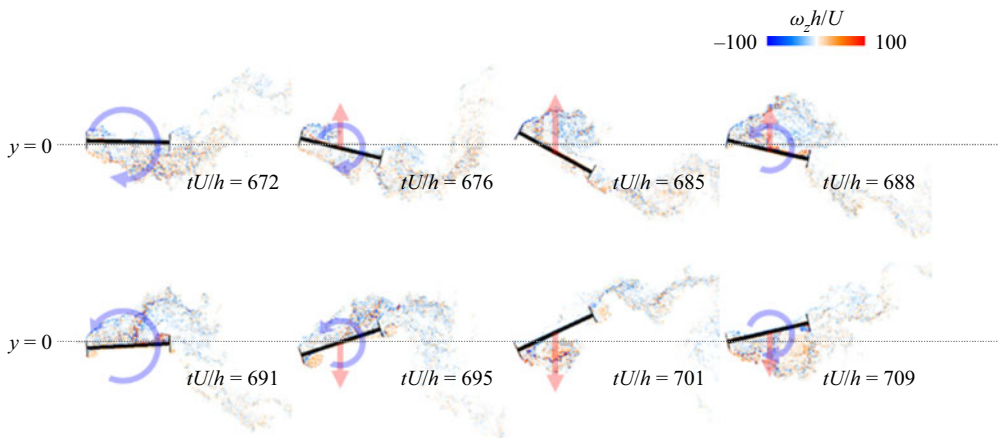
Figure 12. Motion of the deck at z = L_z/4 during the torsional vibration and its relation with the sectional lift and moment exerted on the deck, together with the contours of the instantaneous spanwise vorticity. Here, the scarlet- and light-blue-coloured arrows indicate relative magnitudes of the sectional lift and moment, respectively.
