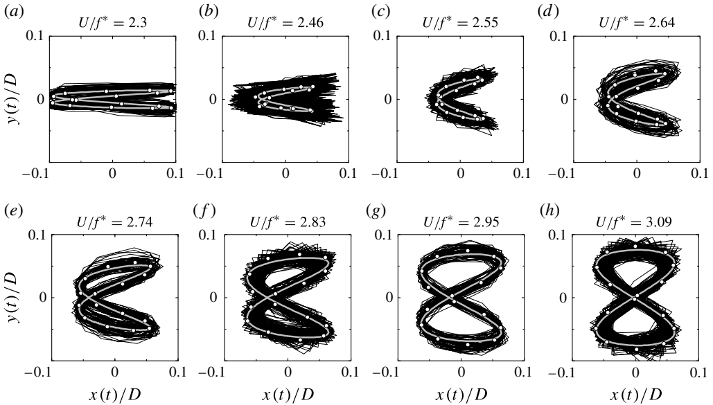
FIGURE 10. The x - y trajectories followed by the cylinder in the reduced velocity range U_r/f^* = 2.3 – 3.1 . The black lines indicate the raw displacement signals, while the white symbols indicate the phase-averaged x and y positions (which were averaged with respect to the y motion) and the thick grey line is a sine-wave fit to the phase-averaged data.
